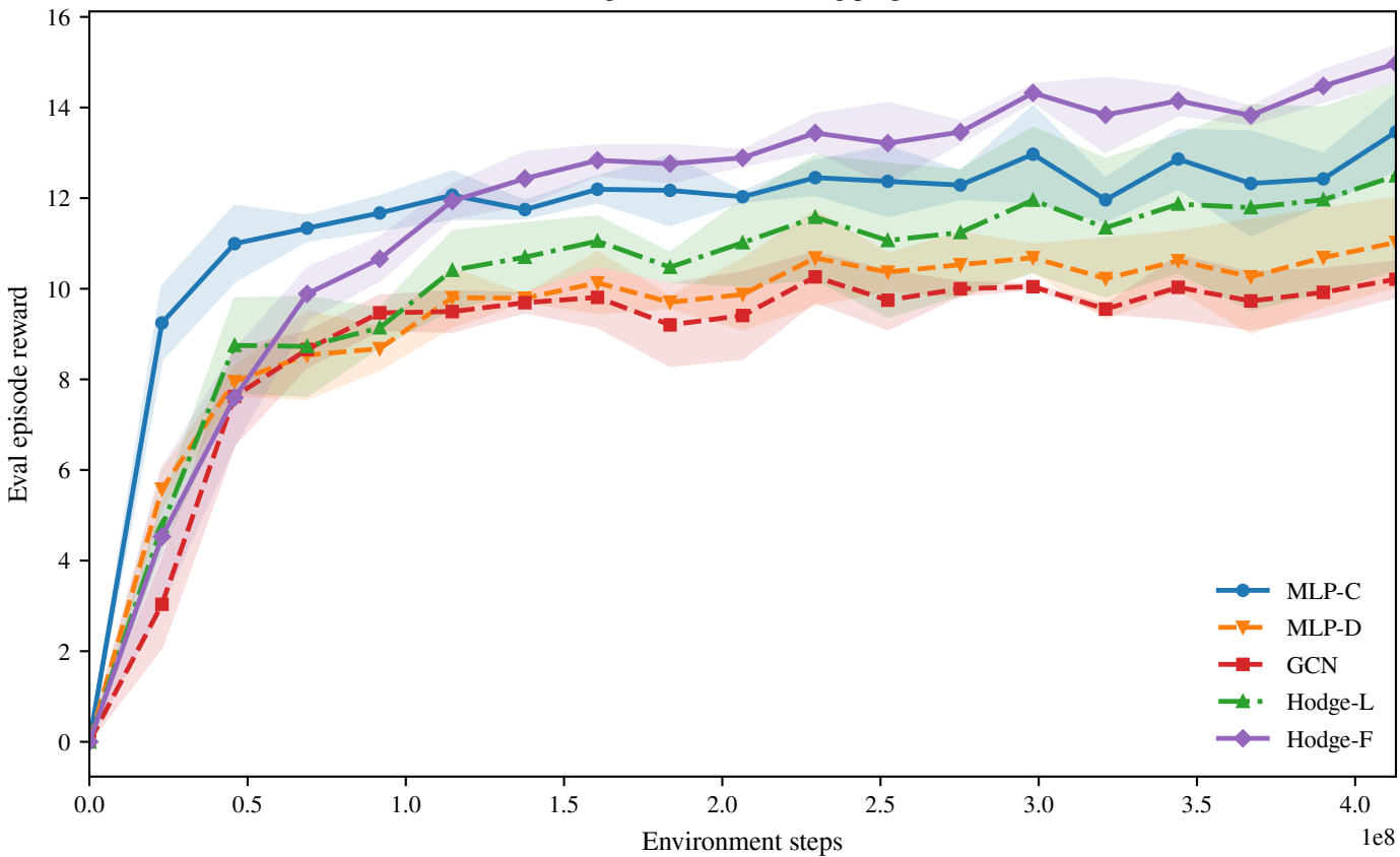
Damage-curriculum training progress
