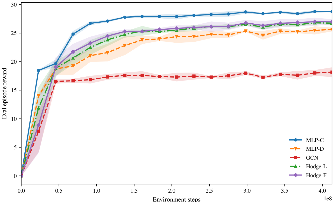
Healthy-only training progress
