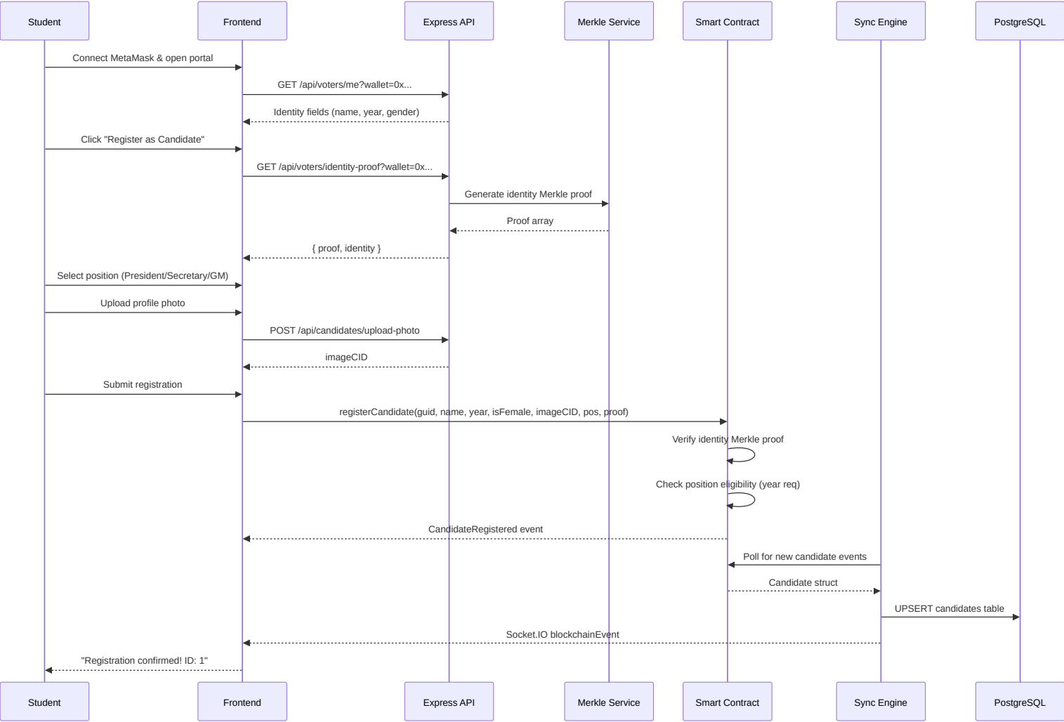
Candidate Self-Registration — Sequence Diagram
