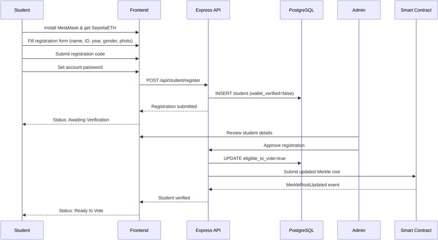
Student Registration — Sequence Diagram
