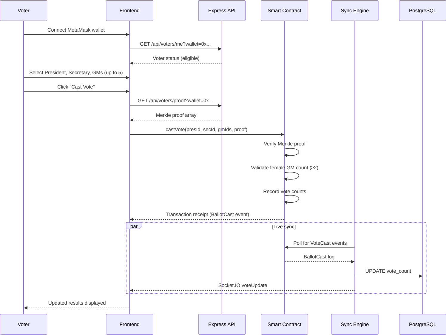
Vote Casting — Sequence Diagram
