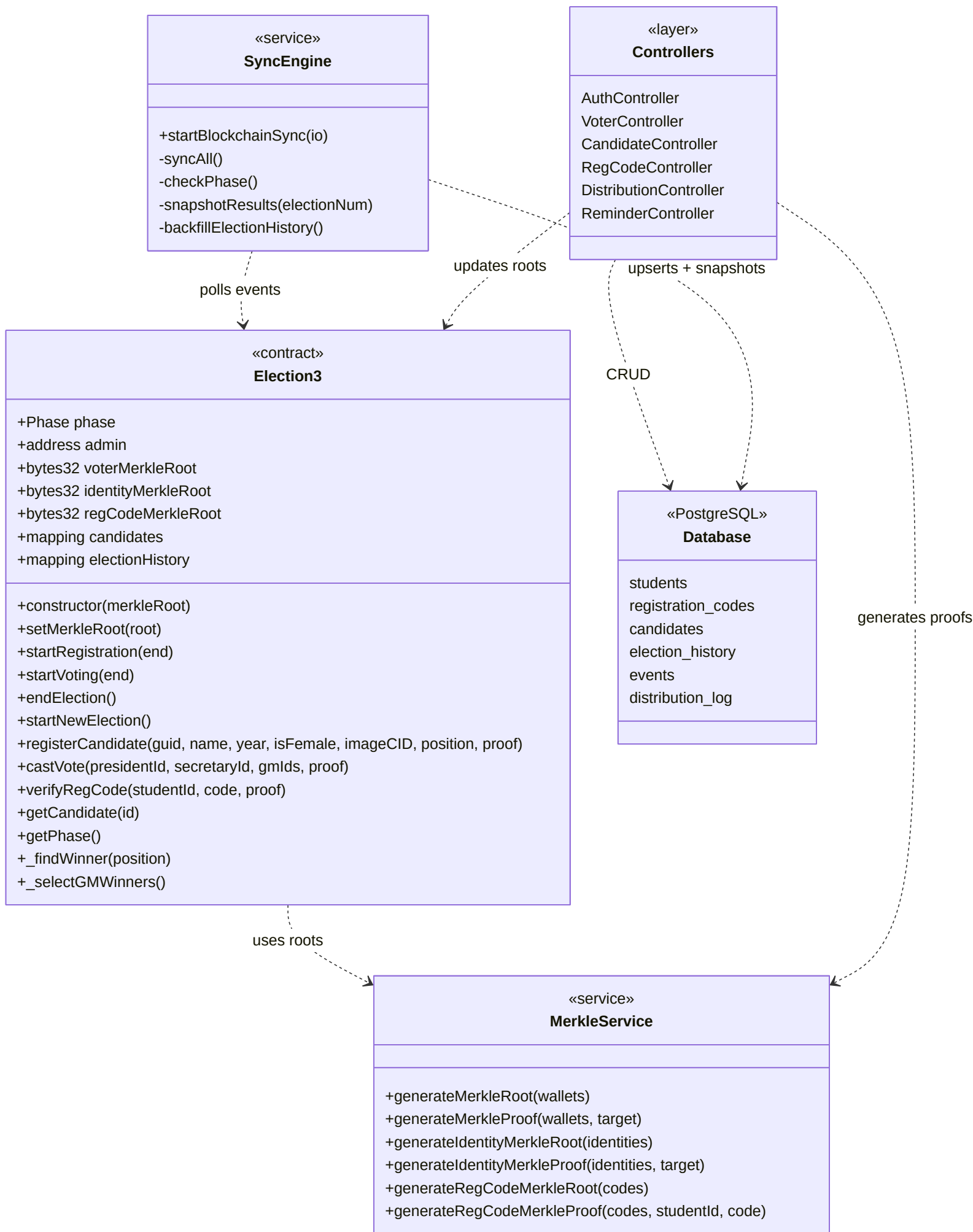
Class Diagram — System Structure
