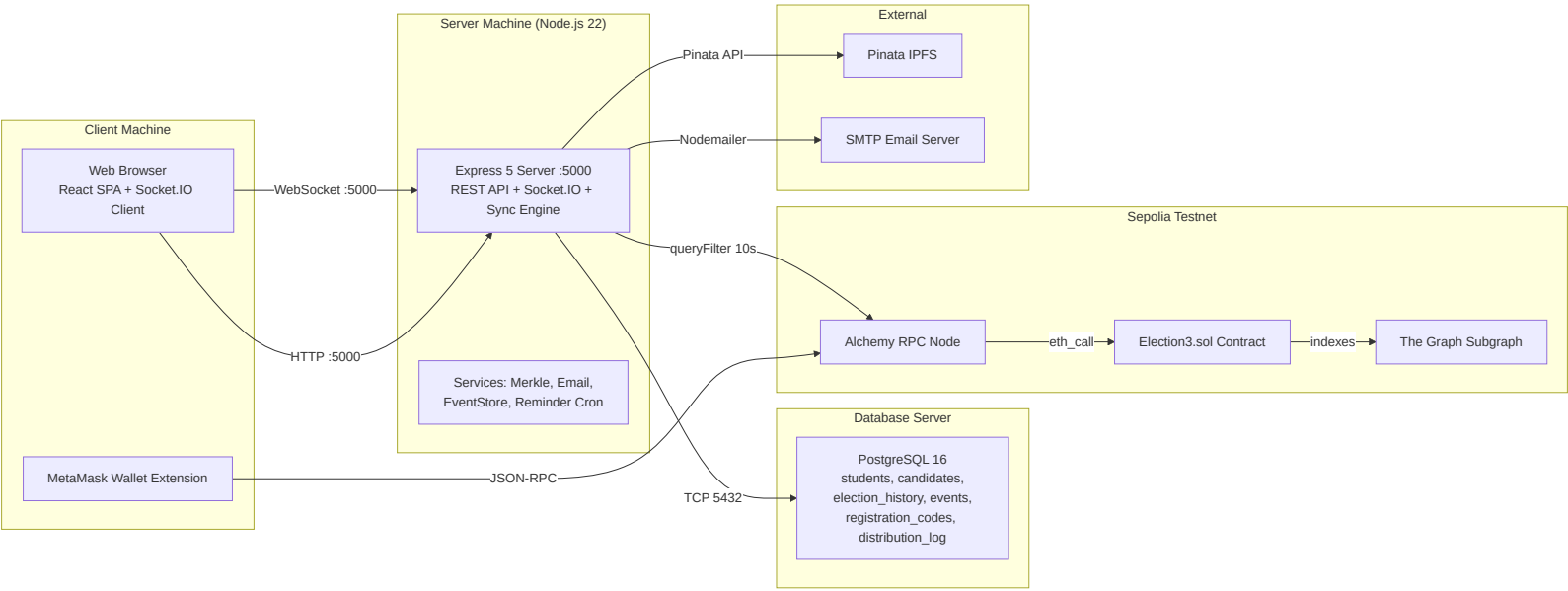
Deployment Diagram — Physical Architecture
