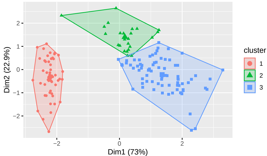
Hierarchical Clusters (k=3)
