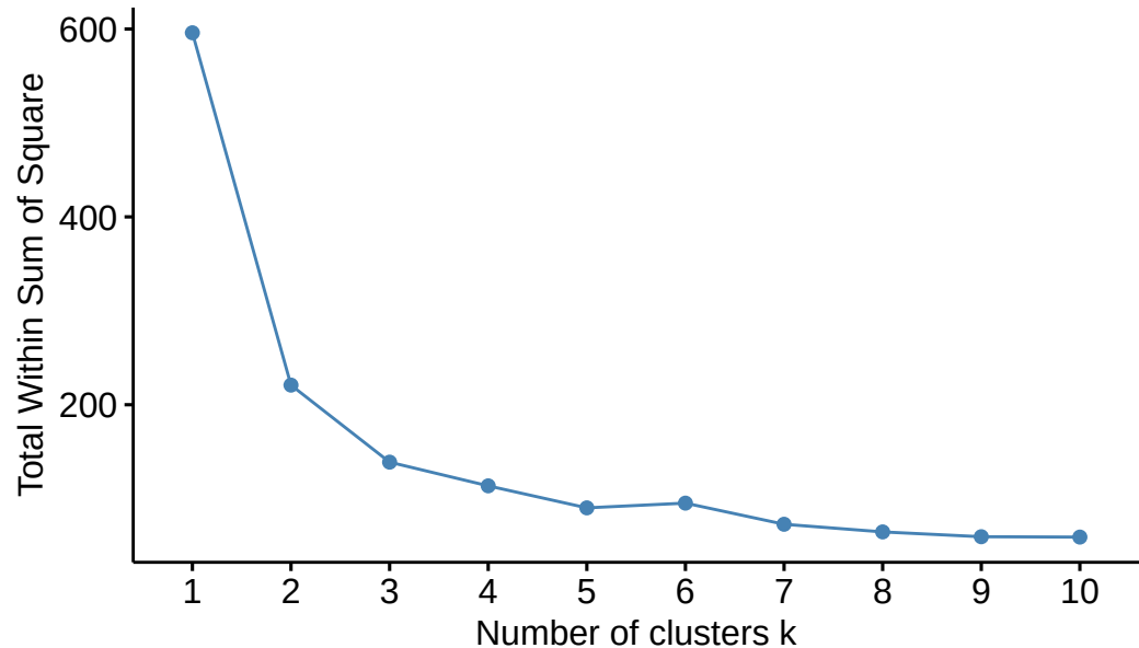
Elbow Method (WSS vs k)
