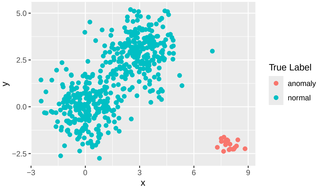
Synthetic Data with Injected Anomalies
