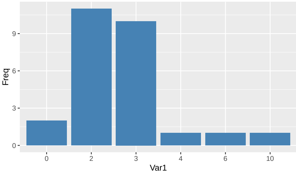
NbClust: Votes for k
