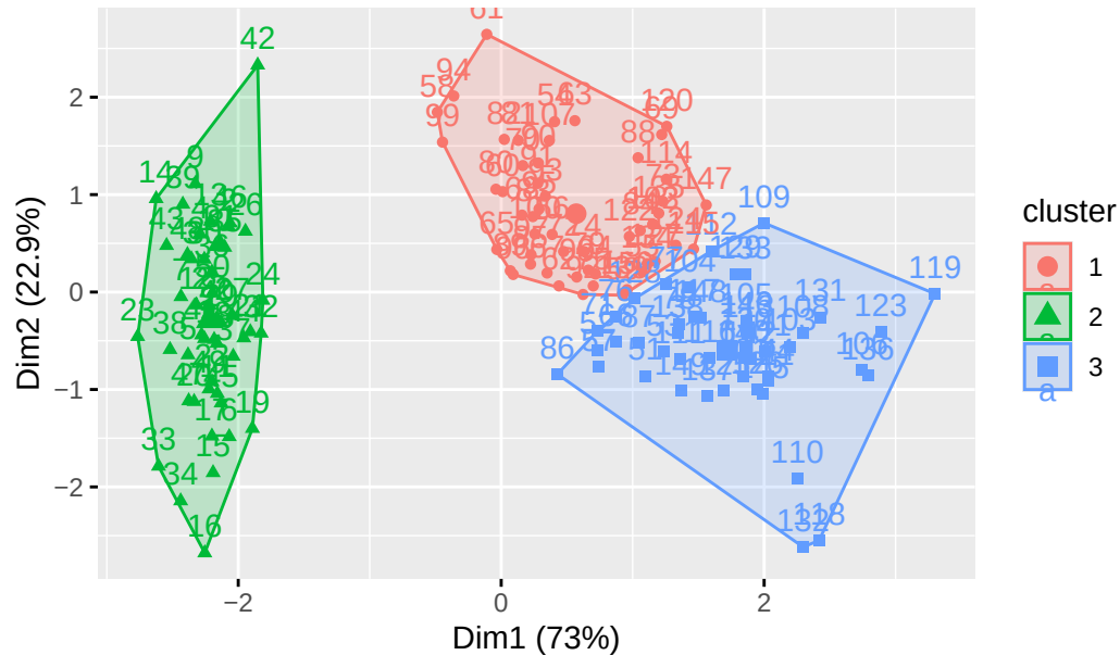
K-means Clusters (k=3)
