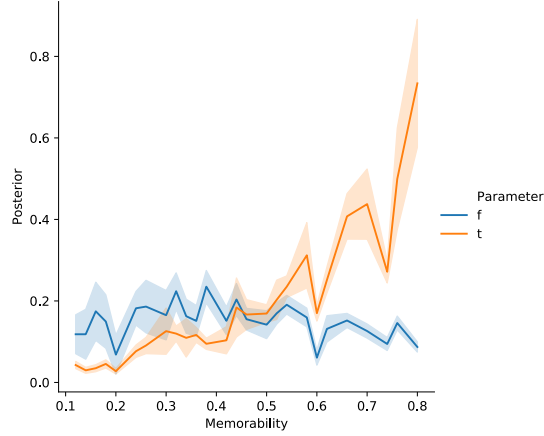
Figure 2.5: Posterior mean \pm 1 SD for f_w and t_w parameters as a function of the word-pair memorability at a three-day delay
