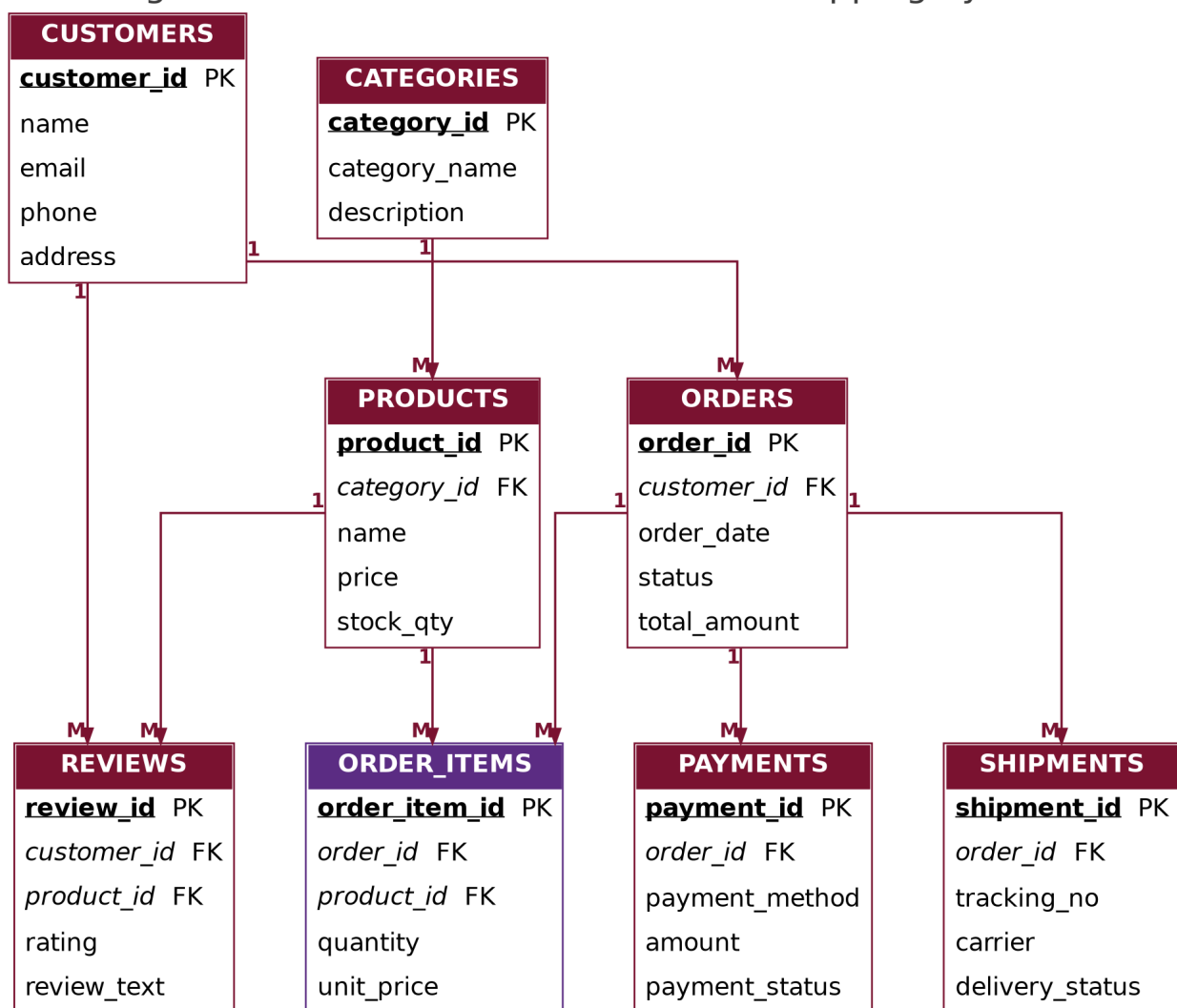
Figure 2 — Relational Schema of the Online Shopping System, showing primary and foreign keys.
