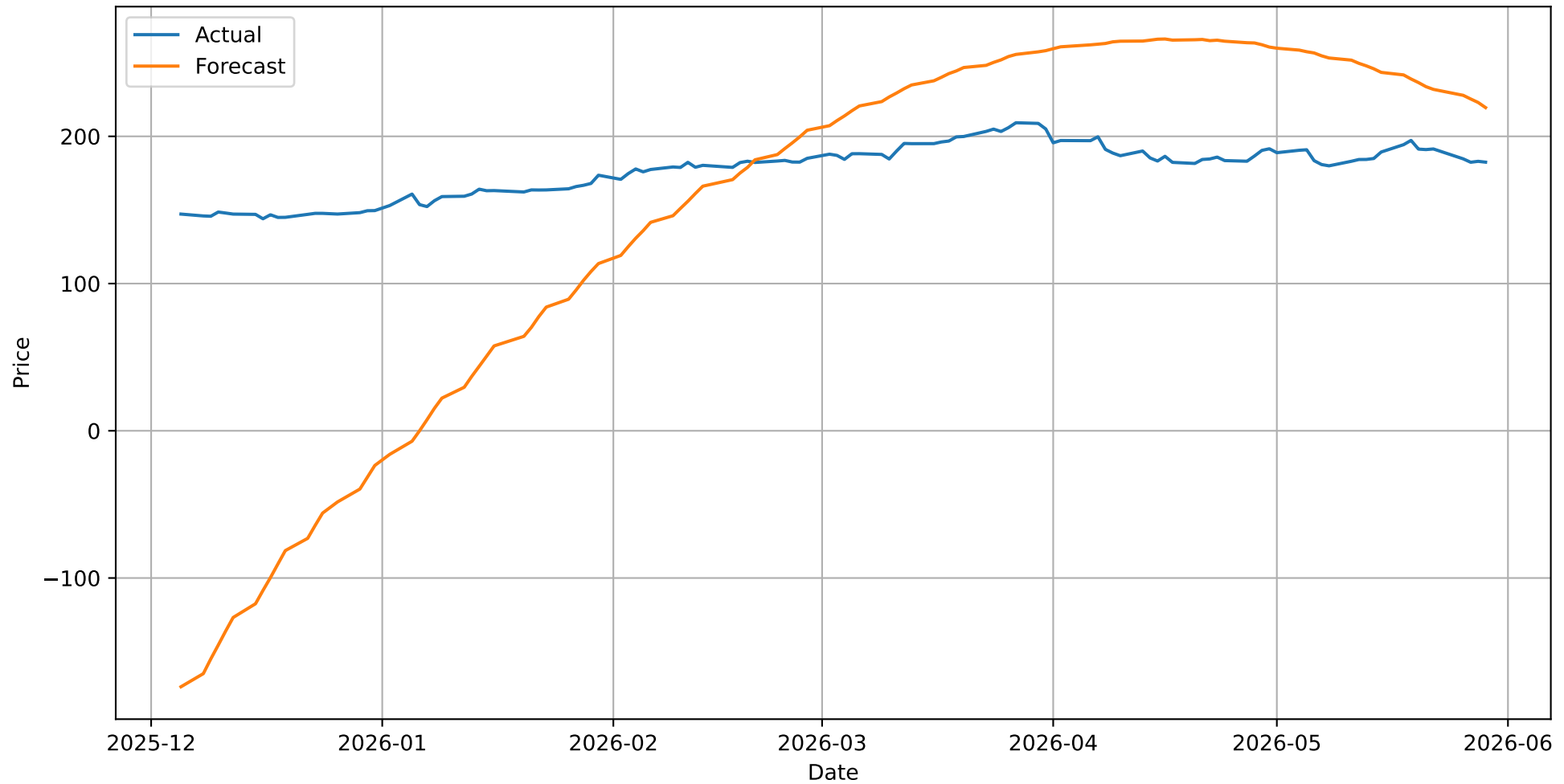
CVX Forecast
