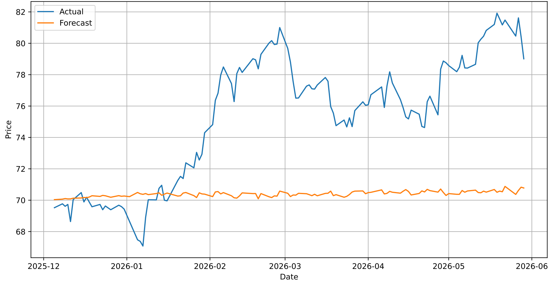
KO Forecast
