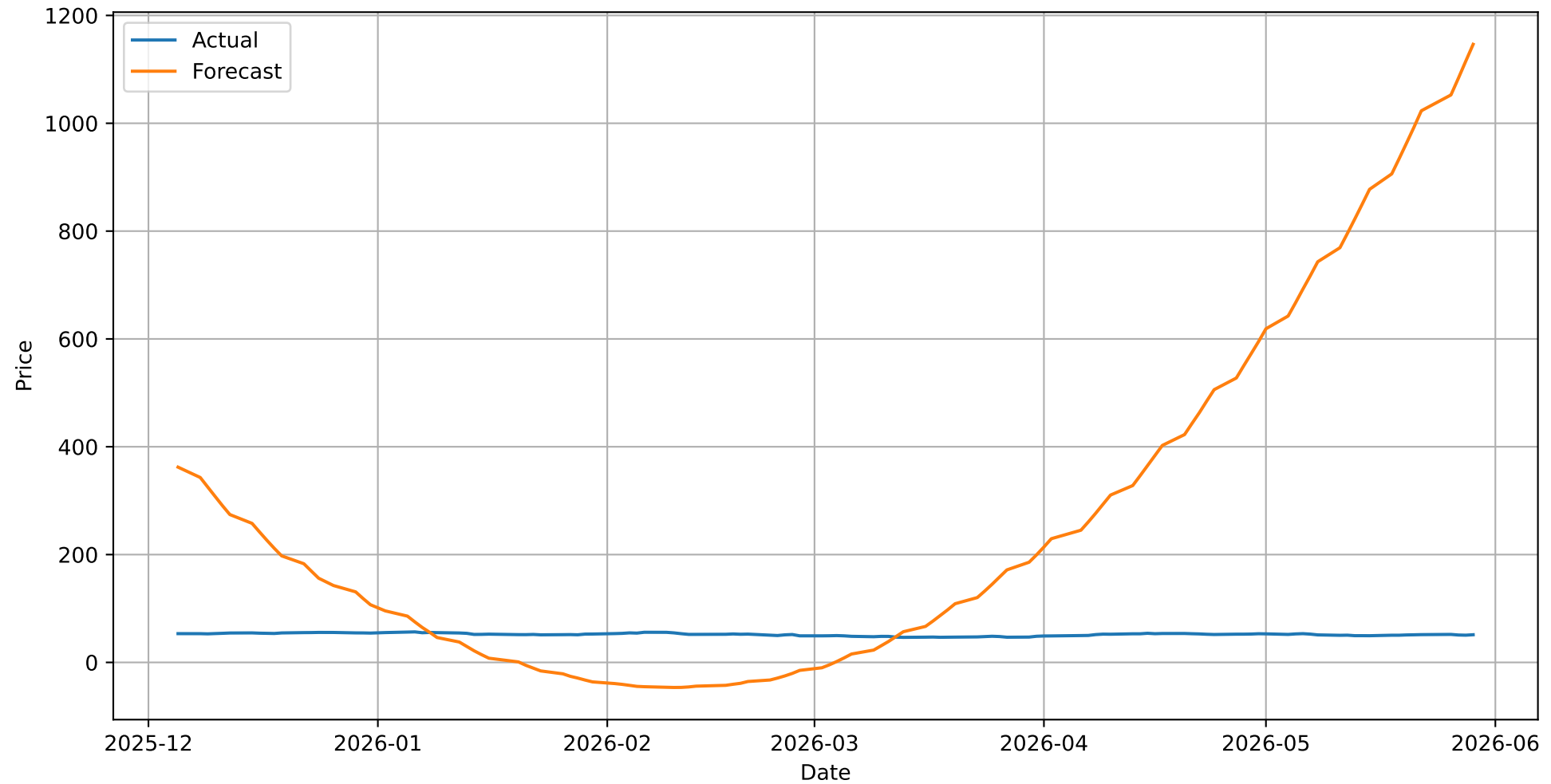
BAC Forecast
