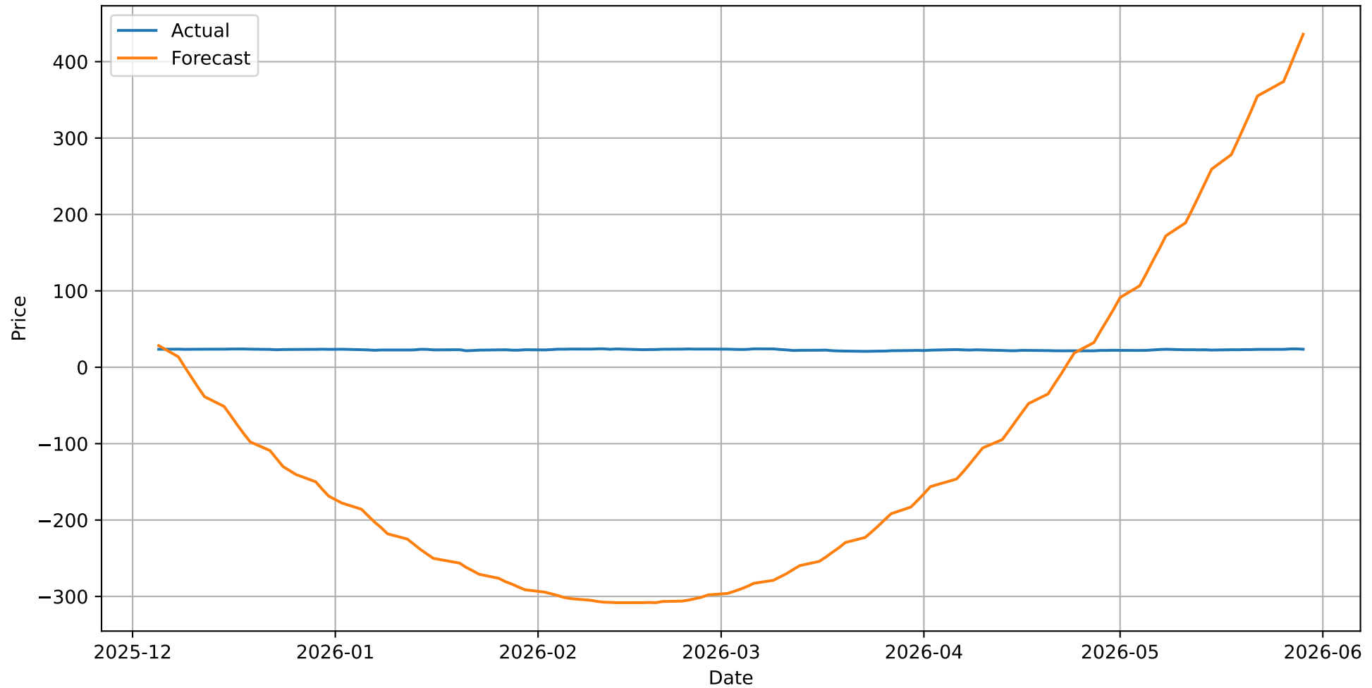
KHC Forecast
