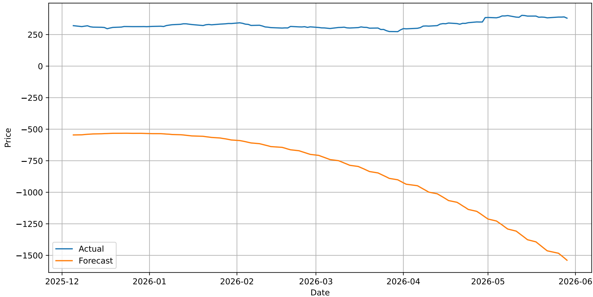
GOOGL Forecast
