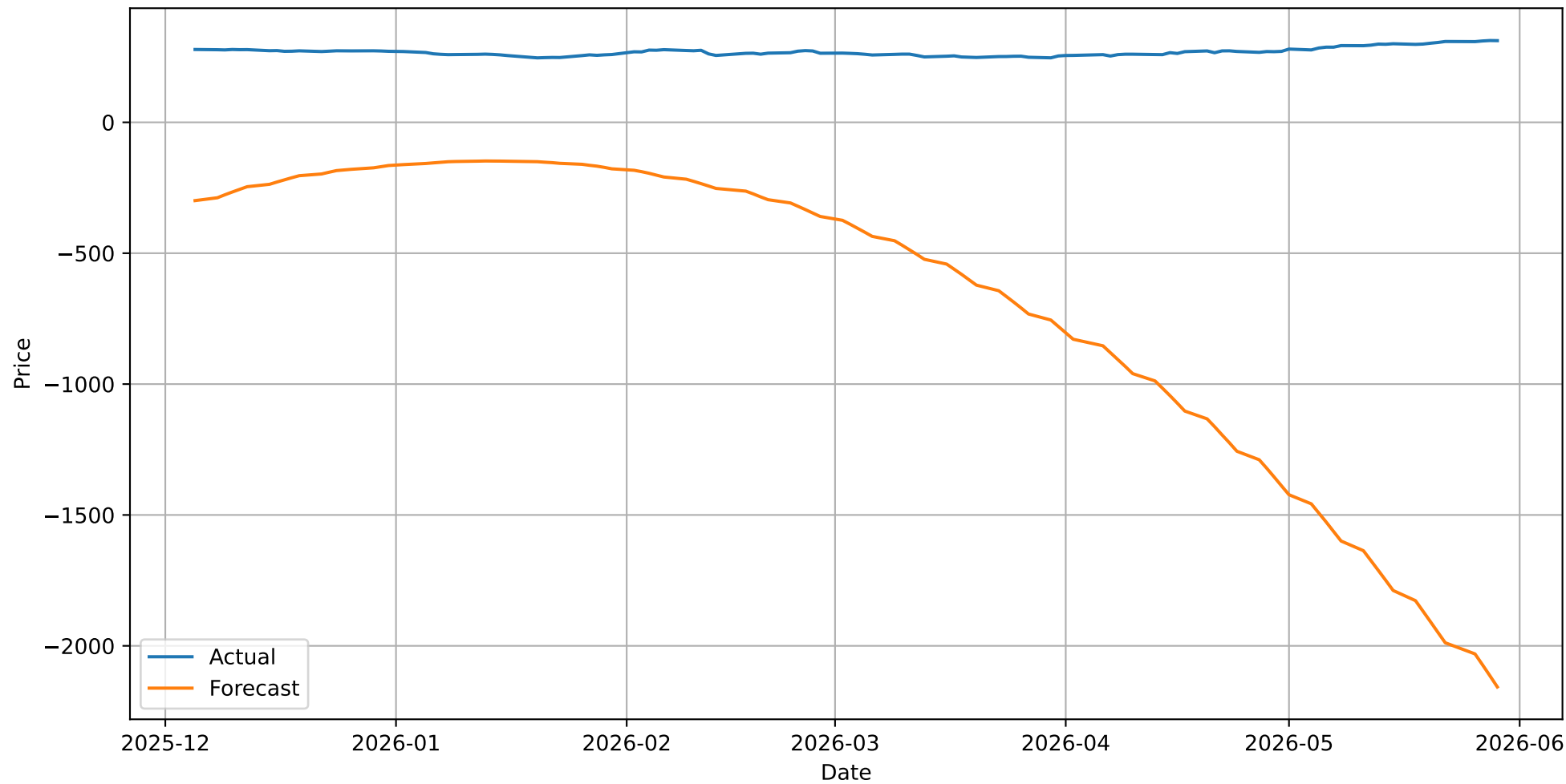
AAPL Forecast
