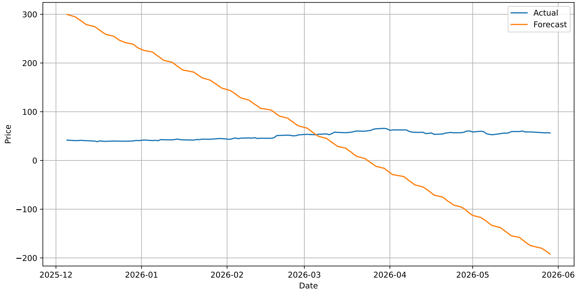
OXY Forecast
