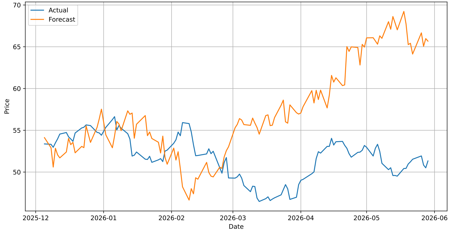
BAC Forecast
