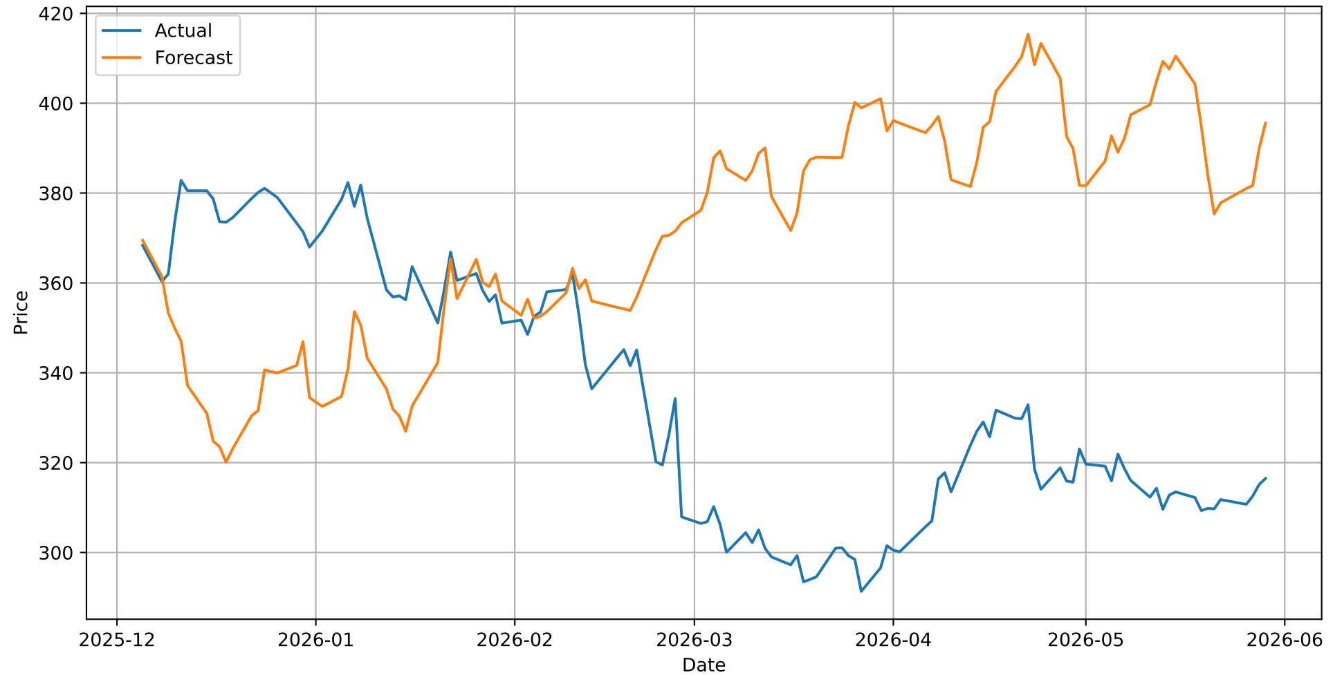
AXP Forecast
