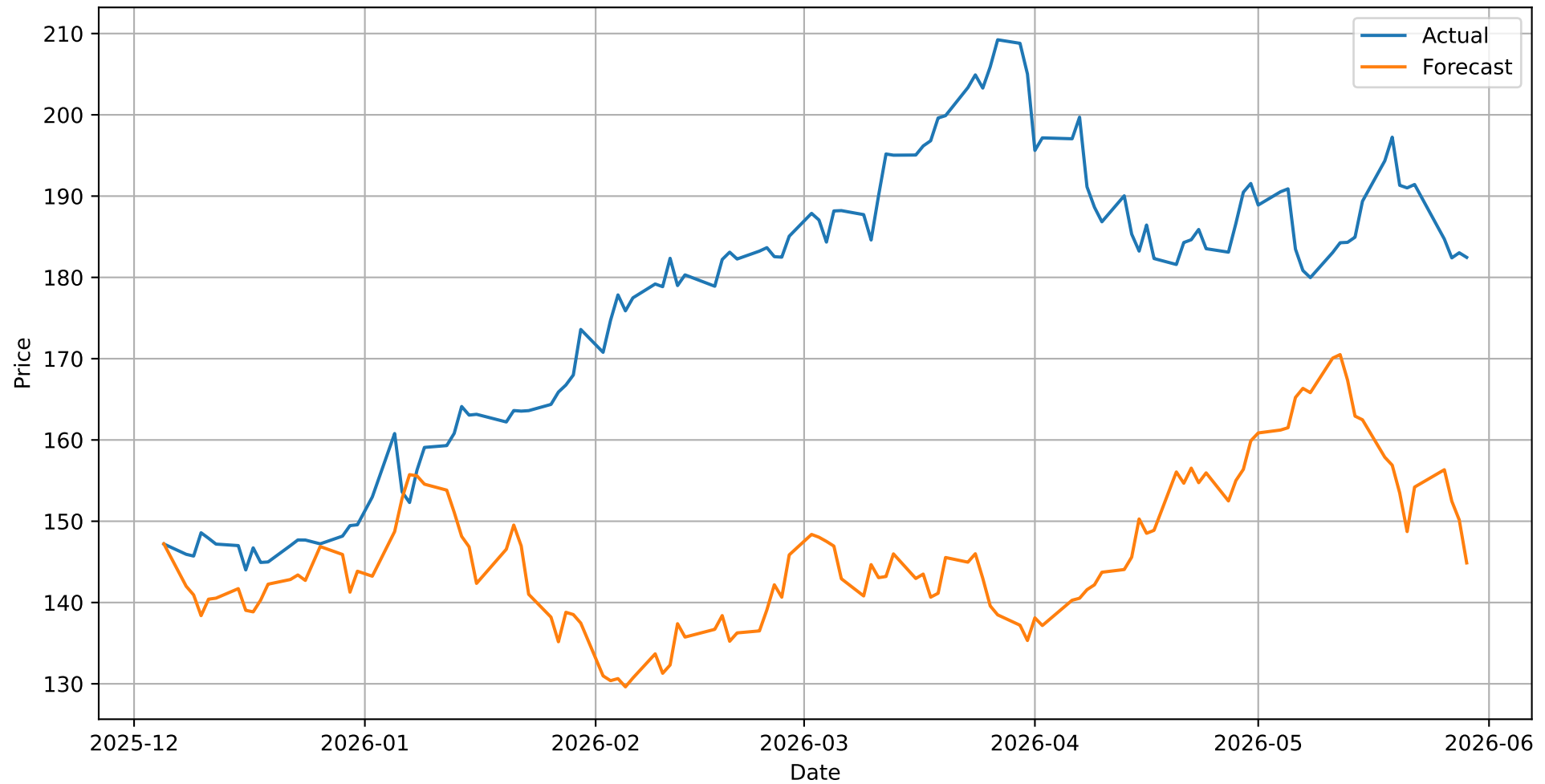
CVX Forecast
