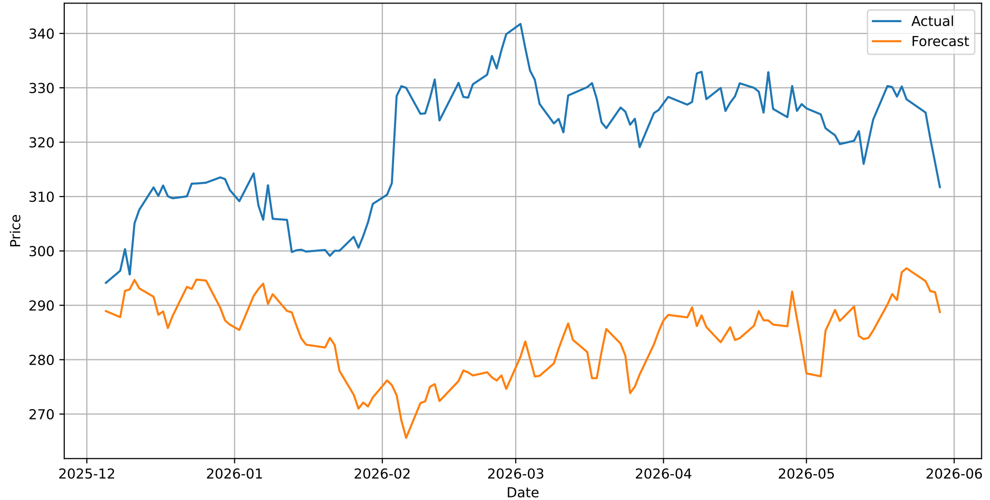
CB Forecast
