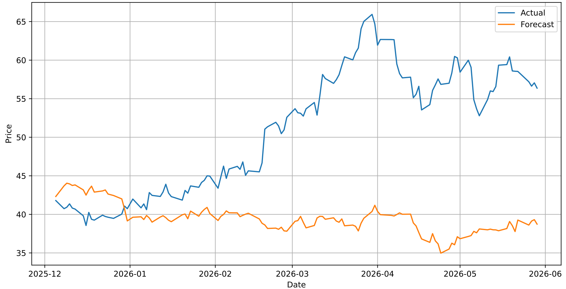
OXY Forecast
