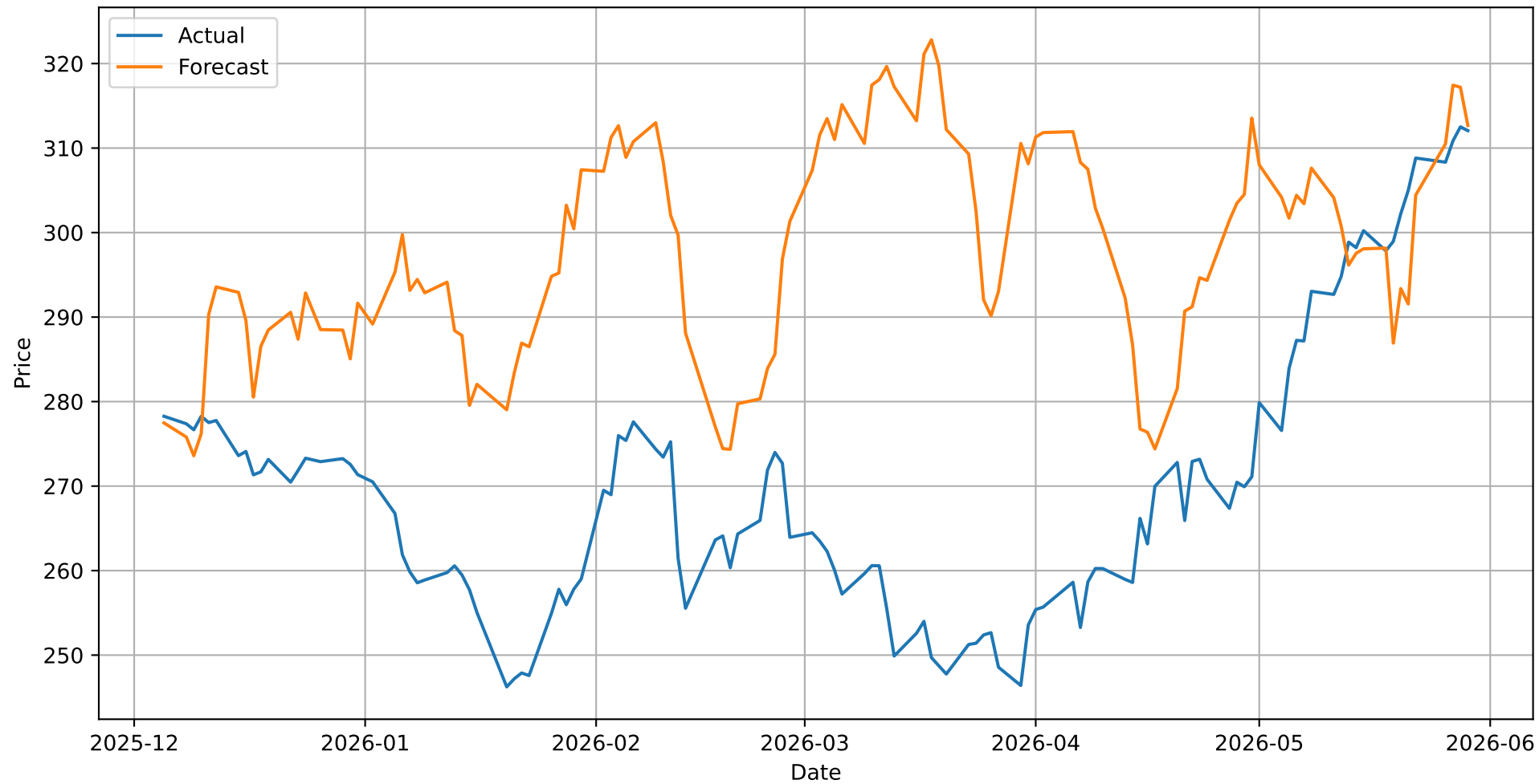
AAPL Forecast
