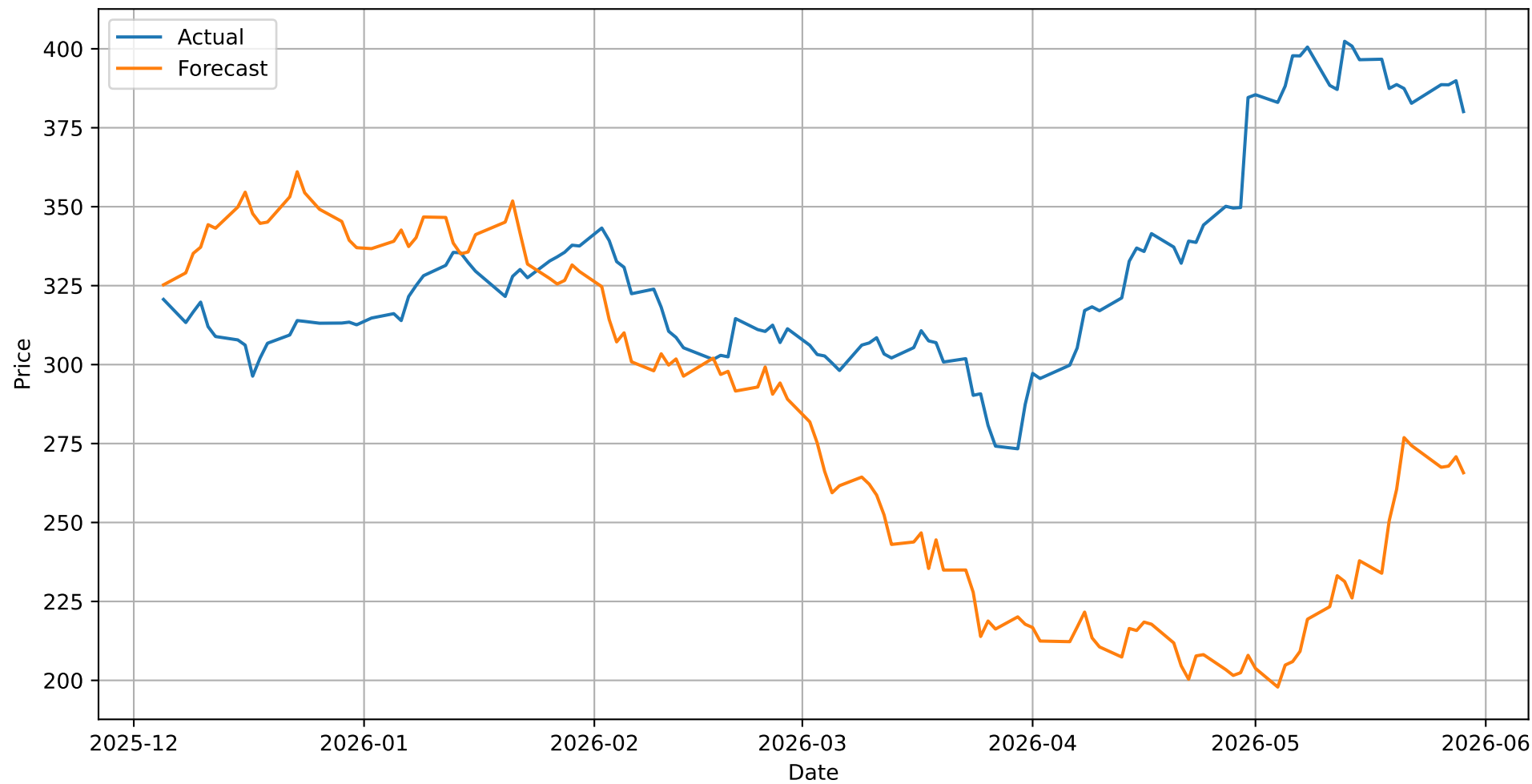
GOOGL Forecast
