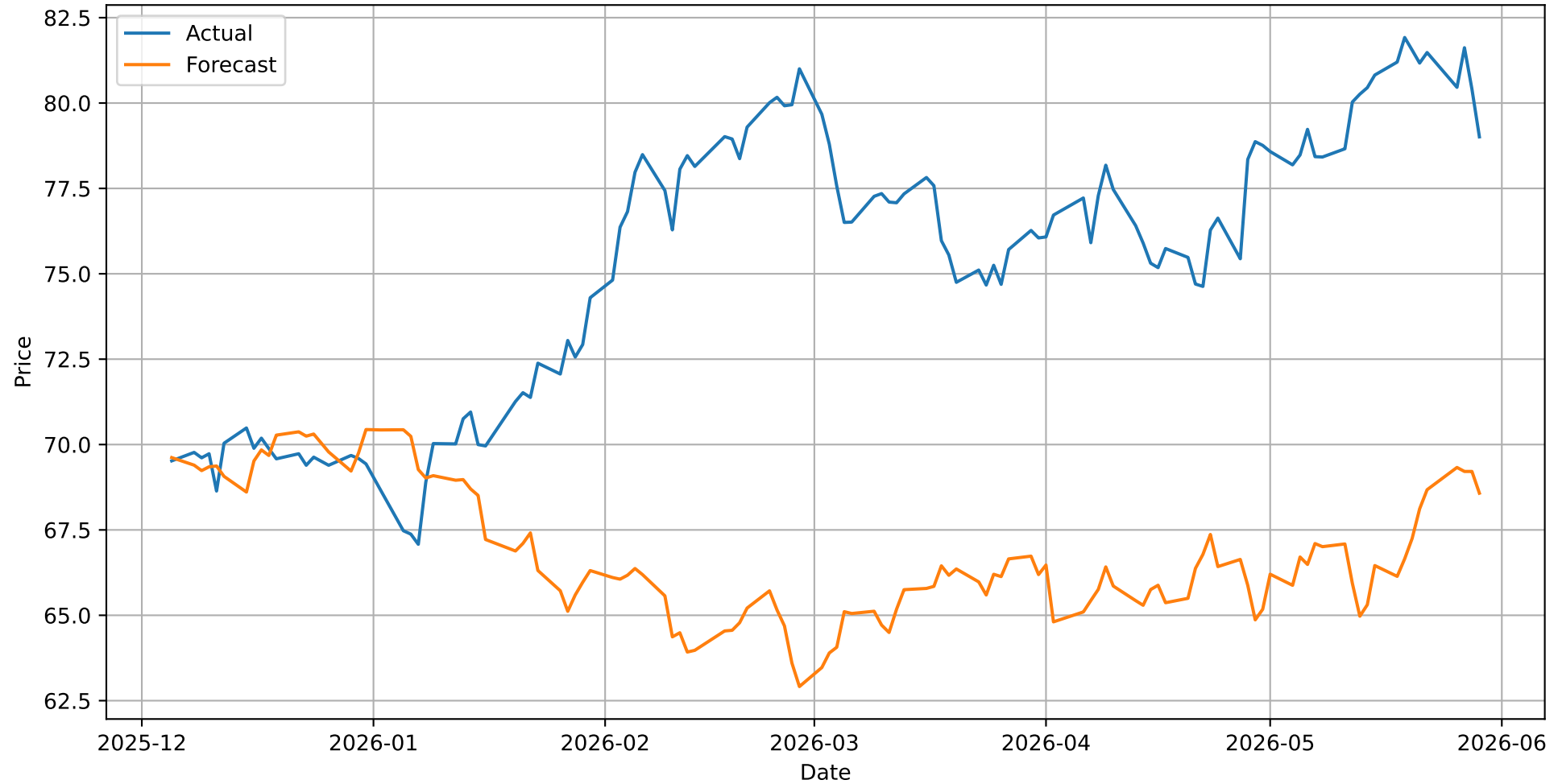
KO Forecast
