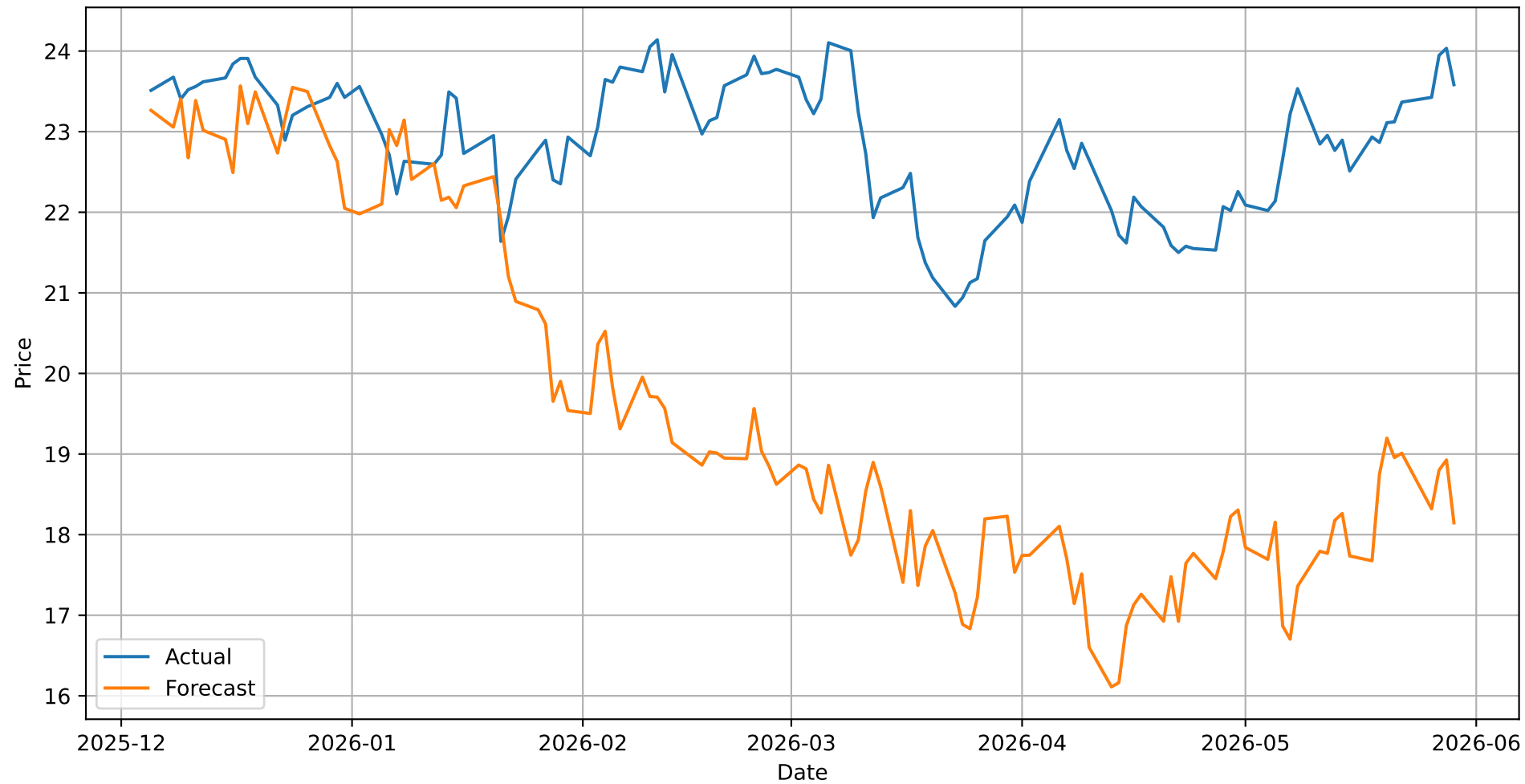
KHC Forecast
