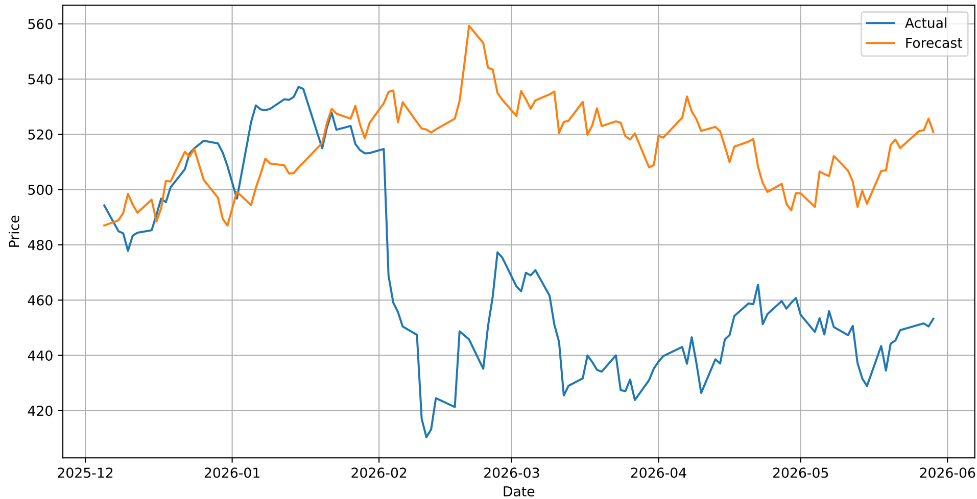
MCO Forecast
