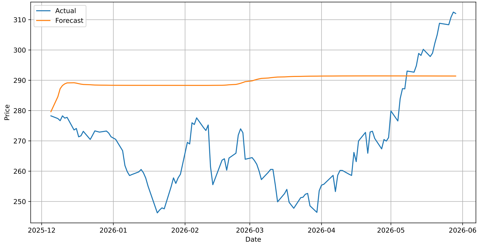
AAPL Forecast
