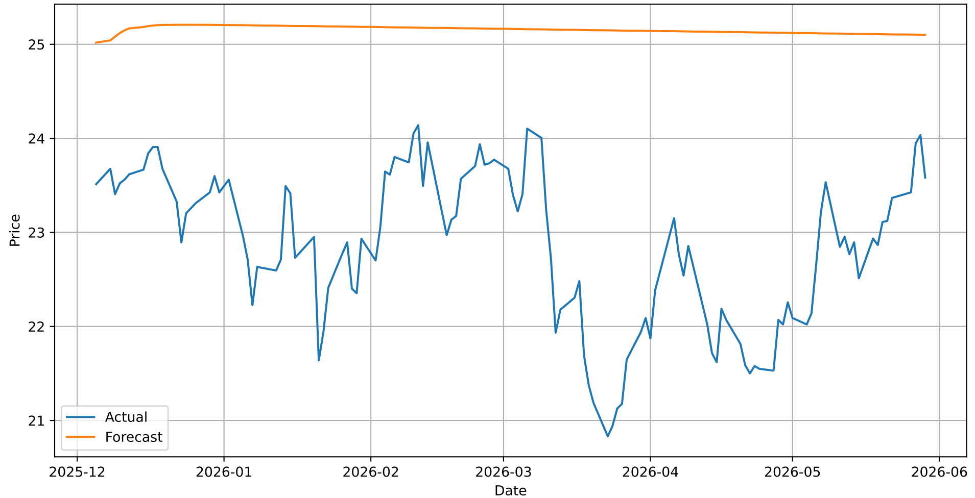
KHC Forecast
