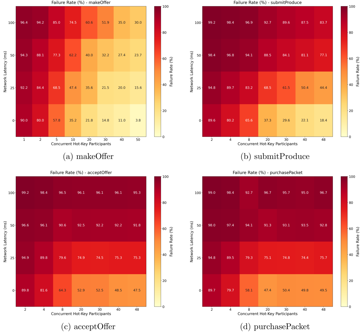
Figure 9: Failure rate matrices for the four core functions at exactly 50 TPS, mapping the interaction between network latency, concurrent hot-key participants, and transaction failure rate.
