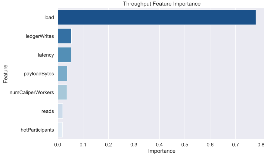
Fig. 9. Random Forest Feature Importance ranking the dominant variables that constrain successful transaction throughput.
