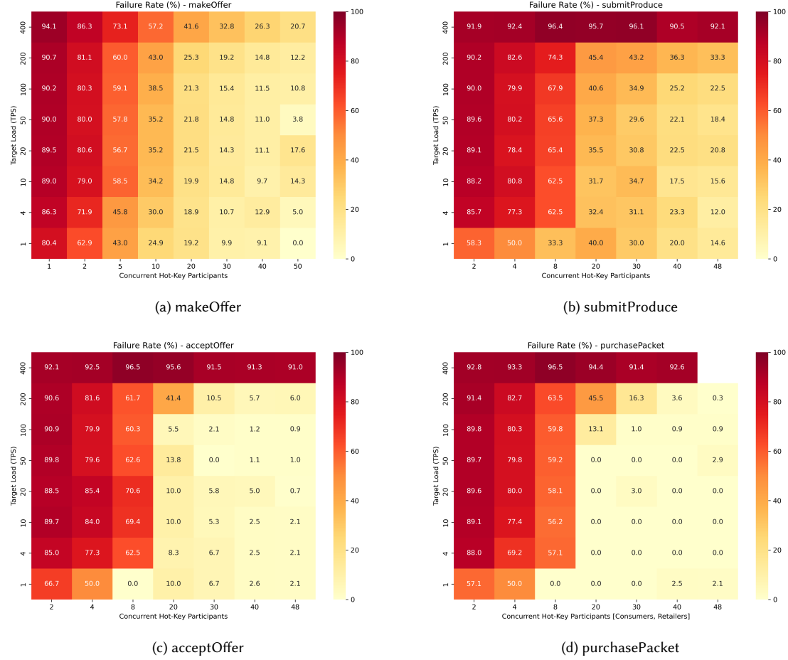
Fig. 6. Failure Rate Danger Zone matrices for the four core functions, mapping the non-linear boundaries of transaction timeouts across Target Load (TPS) and Concurrent Hot-Key Participants.
