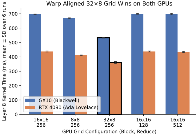
Fig. 3. GPU Layer 8 kernel time by grid configuration, mean \pm SD over 6 runs. The warp-aligned 32 \times 8 grid (outlined) is fastest on both architectures.
