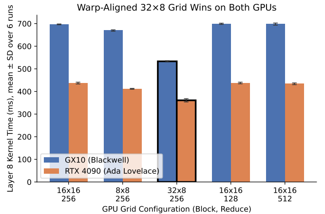
Fig. 1. GPU Layer 8 kernel time by grid configuration on both GPUs, mean \pm SD over 6 runs. The warp-aligned 32\times 8 grid (outlined) is fastest on both architectures, and the advantage is many standard deviations wide on each.
