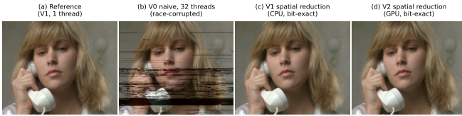
Fig. 1. Frame 26. Panel (b) is one representative V0 run of three on the RTX 4090 (21.5 dB PSNR-Y / 0.767 SSIM against (a)); the scanline artifacts come from unsynchronized writes to img_filt_r_8 . Panels (c) and (d) are pixel-identical to (a) at every configuration tested.
