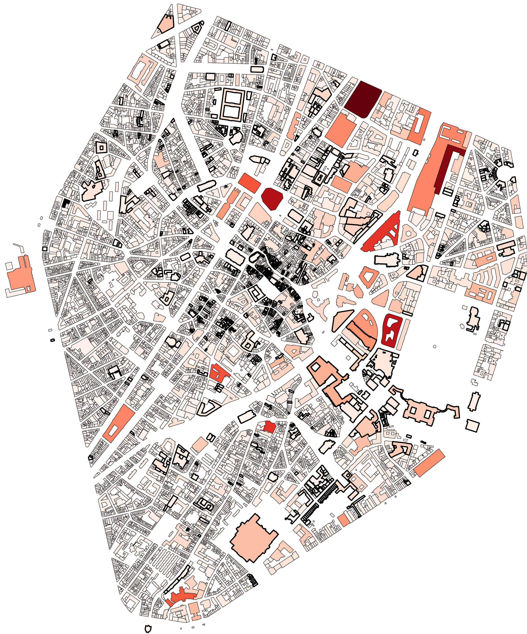
Heating Demand 2020
