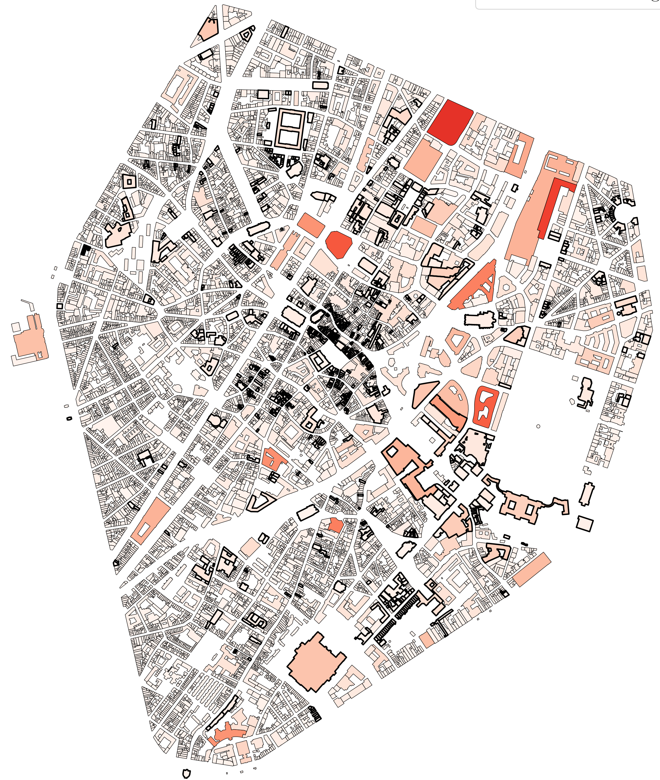
Heating Demand 2050
