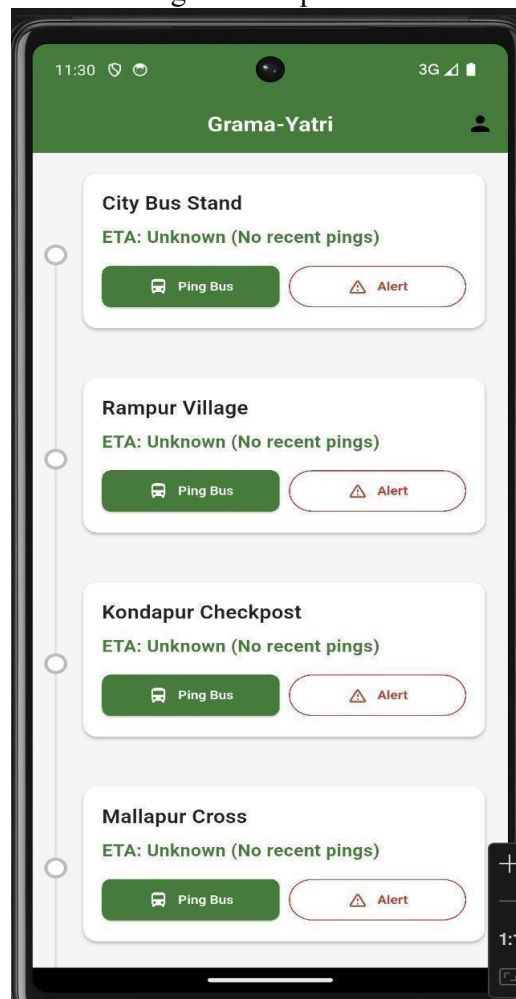
Fig 4.2: User-Interface
