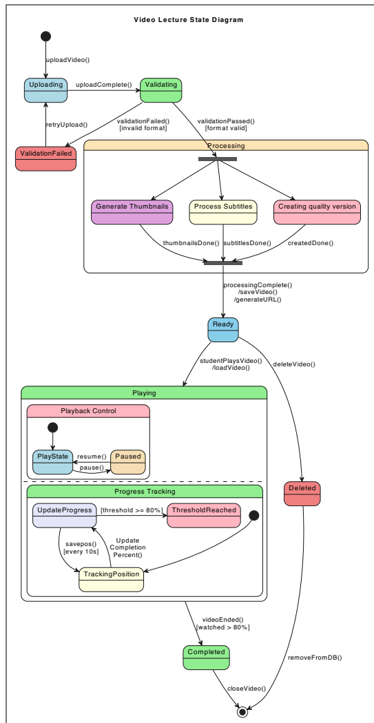
Figure 8.3: Video Lecture Lifecycle
