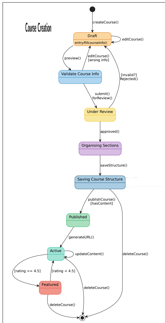
Figure 8.1: Course Creation State Diagram
