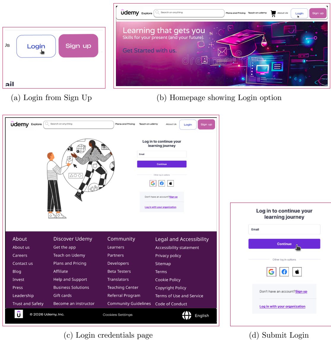
Figure 5.3: Existing User Login Flow
