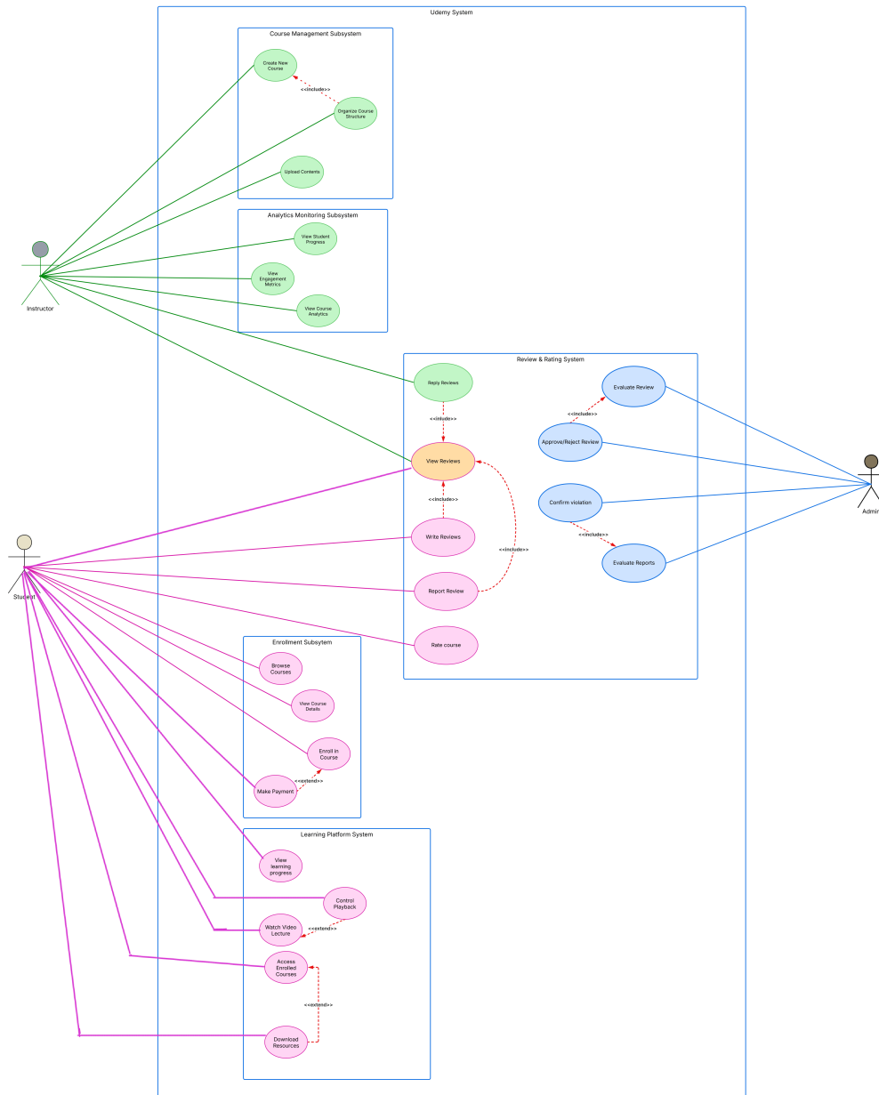
Figure 3.1: Use Case Diagram of the Online Learning Platform Udemy
