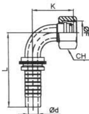
O' RING METRIC FEMALE 24° CONE SEAT H.T - DIN 3865 SERIES 'S' DIN 2353 (SLIP ON NUT) ( EN 856 / 4SP / 4SH )
