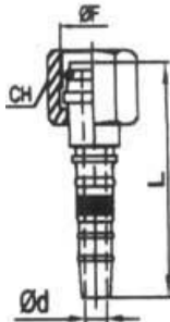
90° 'O' RING METRIC FEMALE ELBOW 24° CONE SEAT H.T - DIN 3865 SERIES 'S' DIN 2353 (SLIP ON NUT) ( SAE100 R13 )
