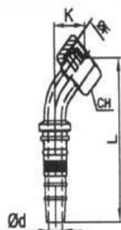
45° 'O' RING METRIC FEMALE ELBOW 24° CONE SEAT H.T - DIN 3865 SERIES 'S' DIN 2353 (SLIP ON NUT) ( SAE100 R13 )
