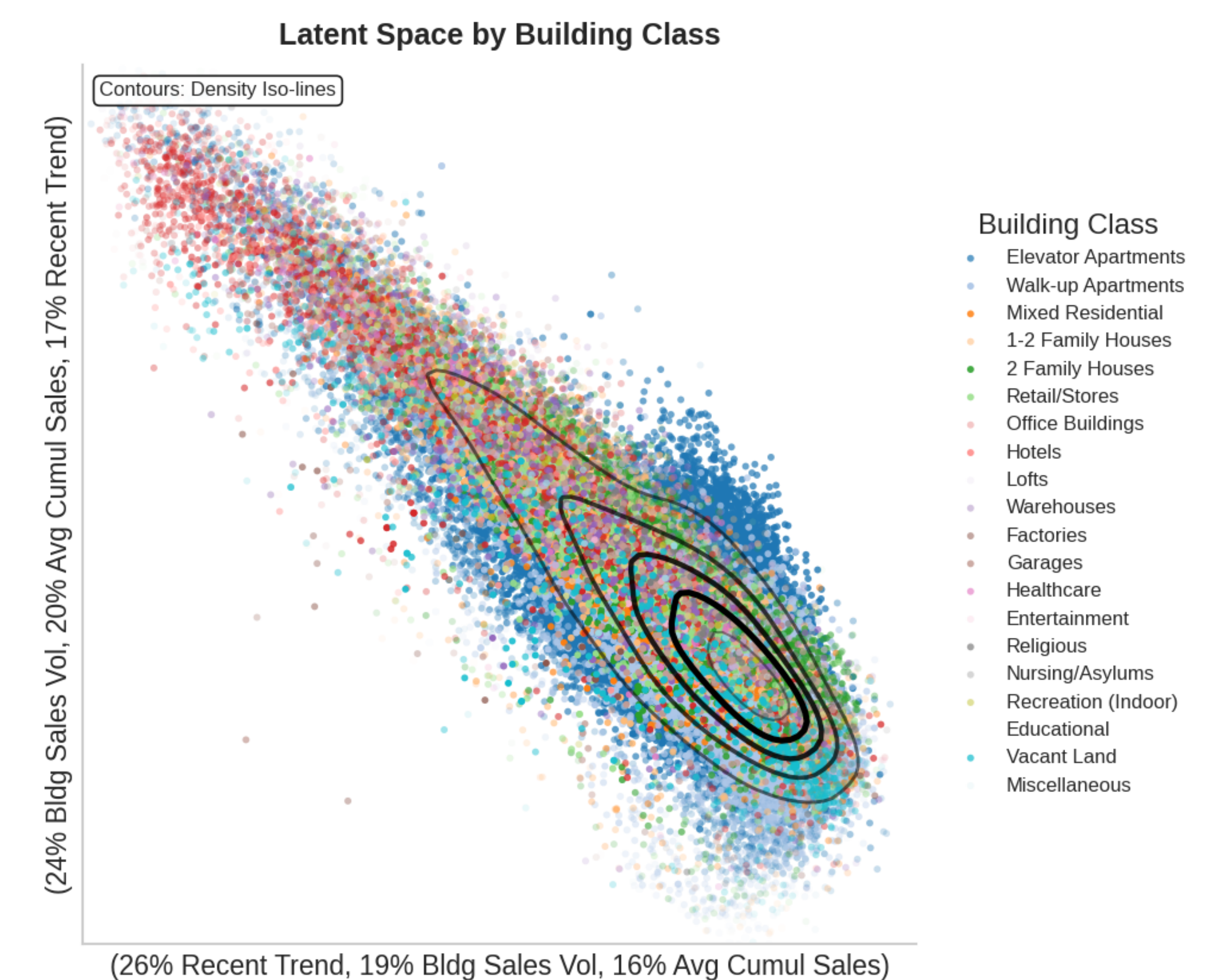
Figure: Latents by Building Class: Identifiable striations.
