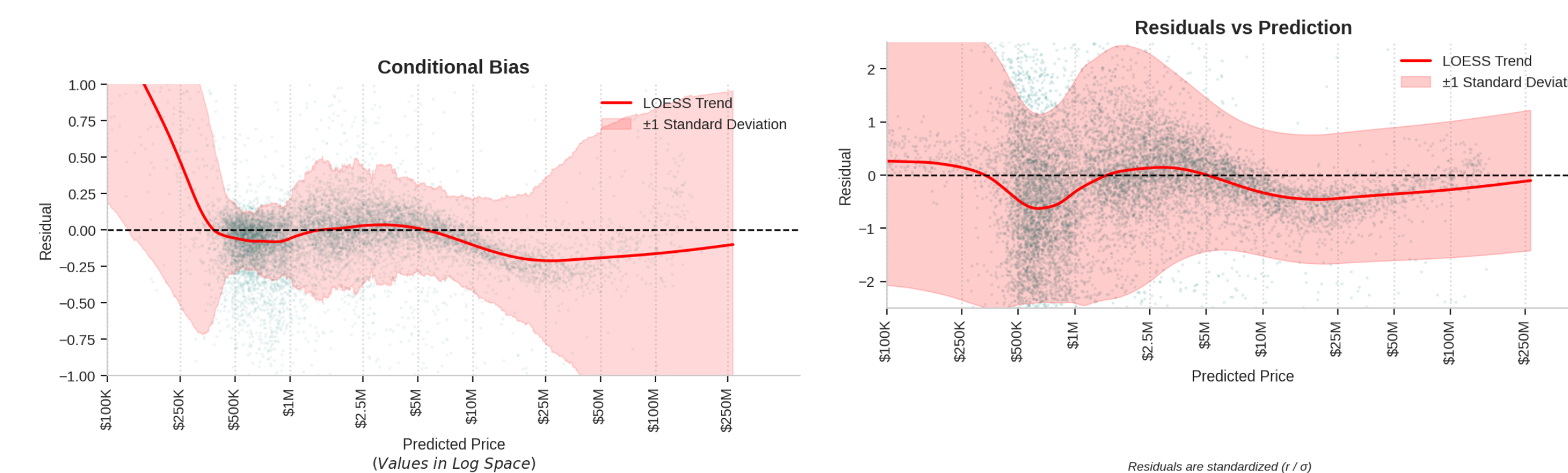
Figure: Model Assumption Checks: Conditional Bias (left) and Homoscedasticity (right).
