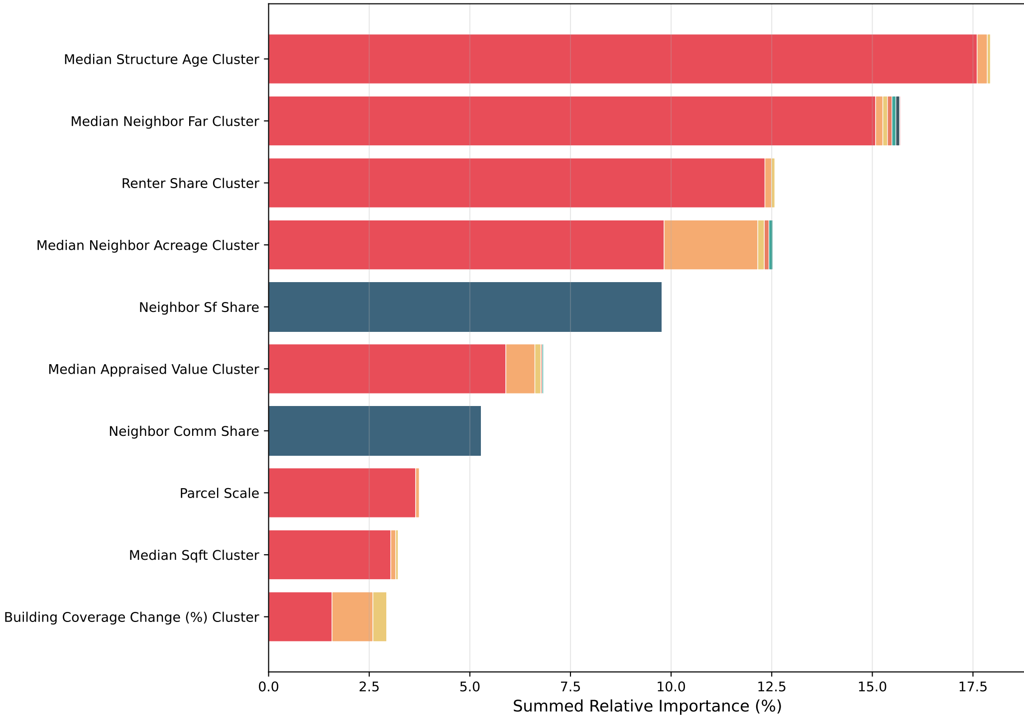
Top 10 Predictor Groups After Correlation Clustering (Filing Date Baseline)
