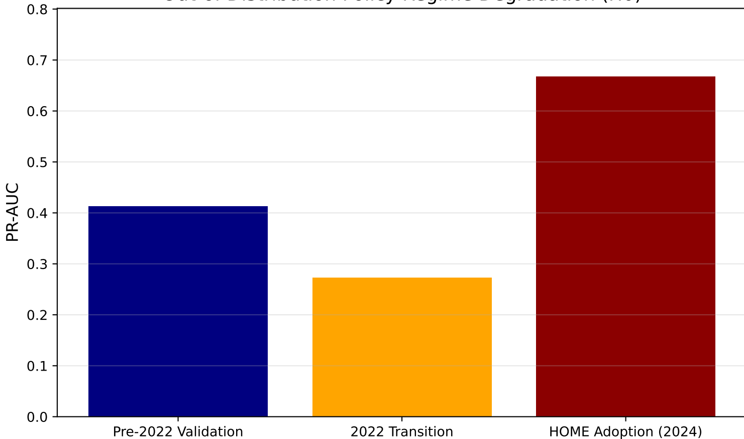
Out-of-Distribution Policy Regime Degradation (H0)
