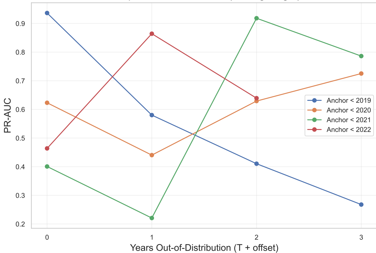
Temporal Predictive Drift (Rolling Origin)
