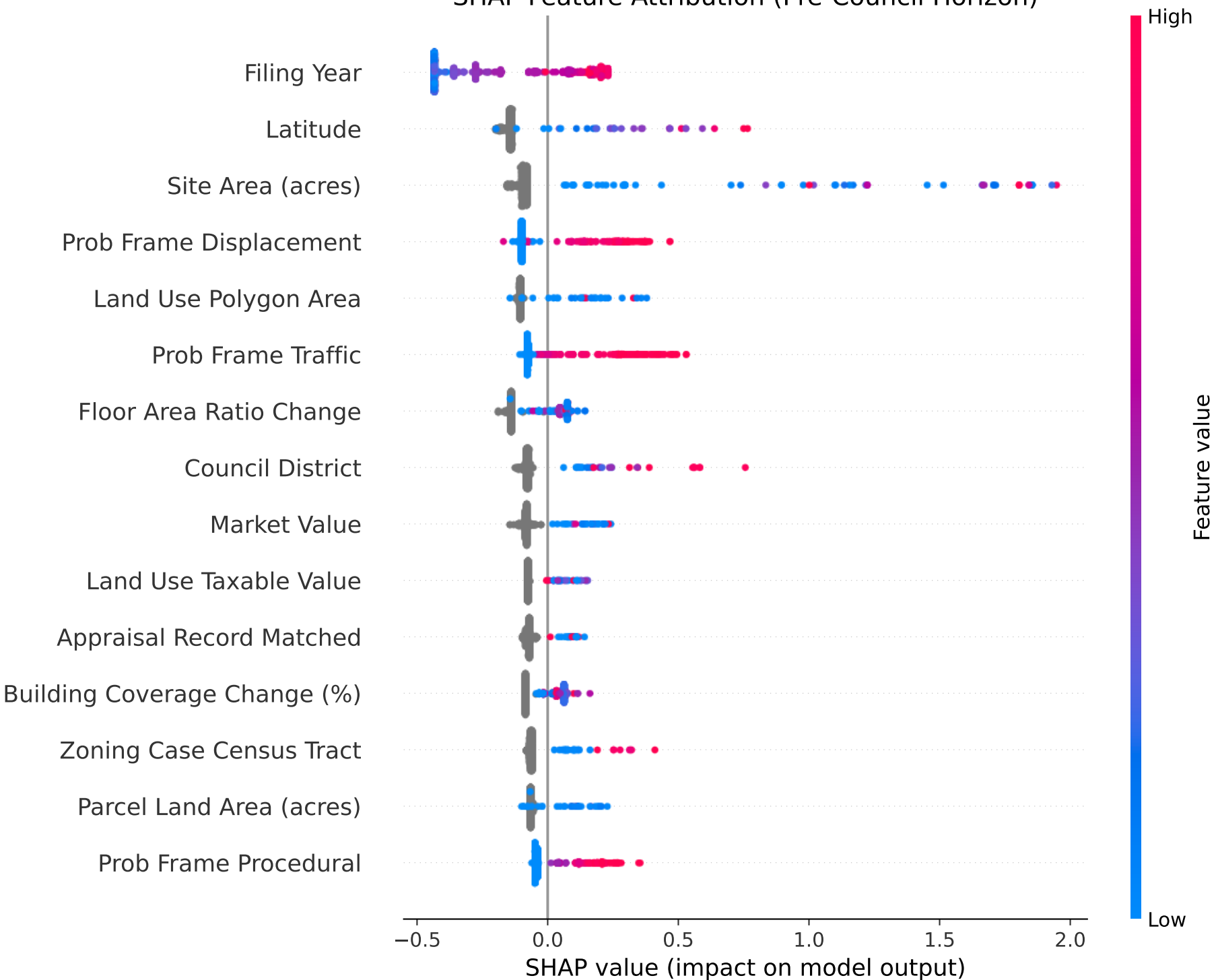
SHAP Feature Attribution (Pre-Council Horizon)
