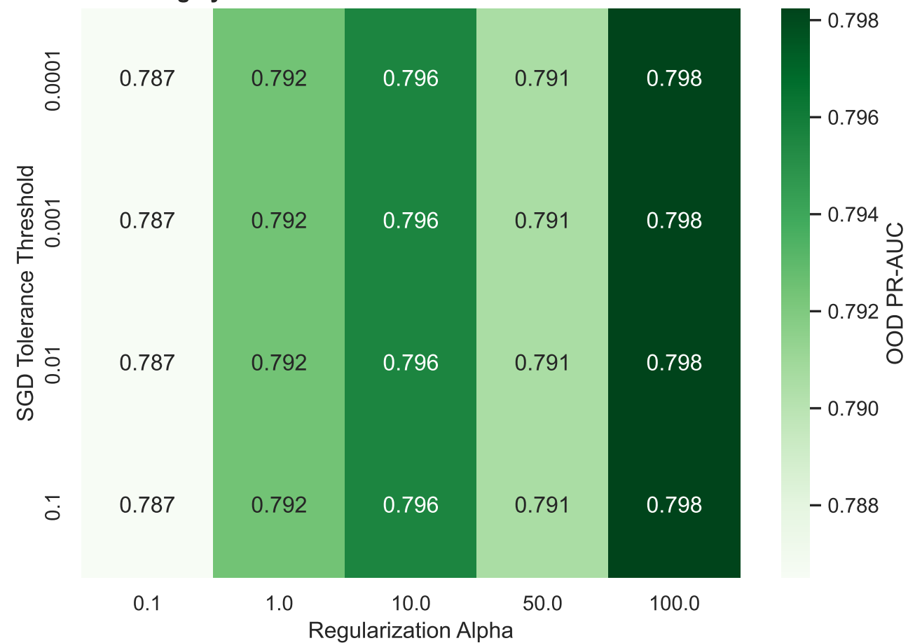
Causal Structures (Ridge) Highly robust continuous constraint boundaries
