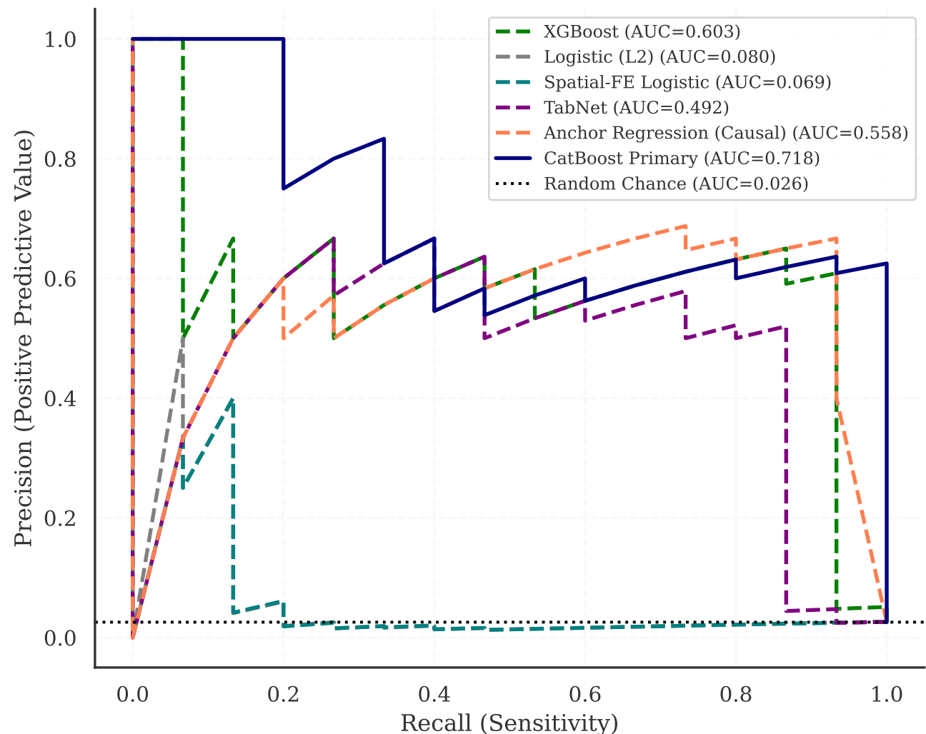
Filing-Date Precision-Recall Curves by Model Class
