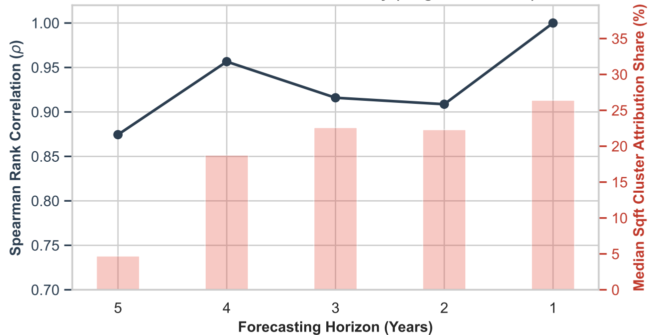
Multi-Horizon Attribution Stability (Target Year: 2023)
