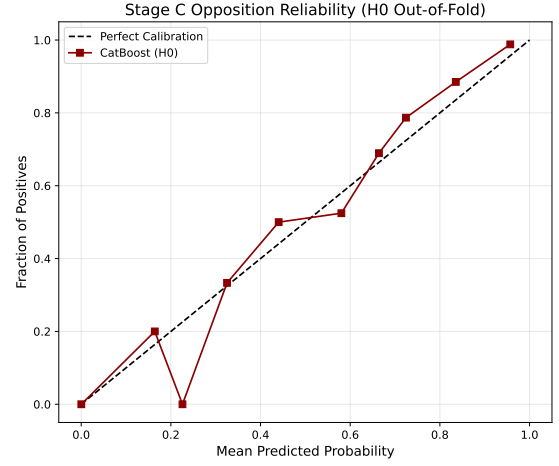
(b) Stage C: Opposition model reliability (ECE = 0.126).
