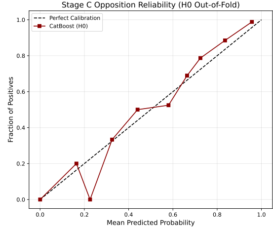
(b) Stage C: Opposition model reliability (ECE = 0.126).
