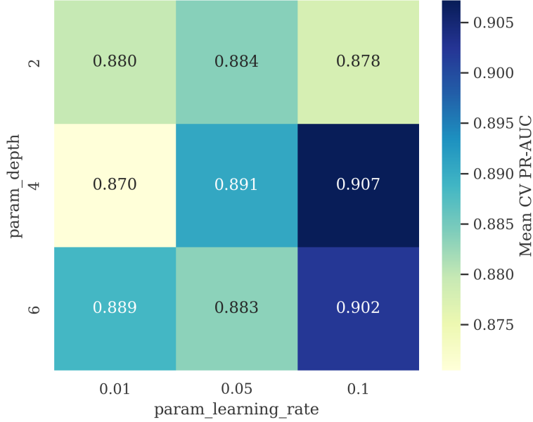
CatBoost Actual GridSearchCV Optimization Surface (H0 Enriched)
