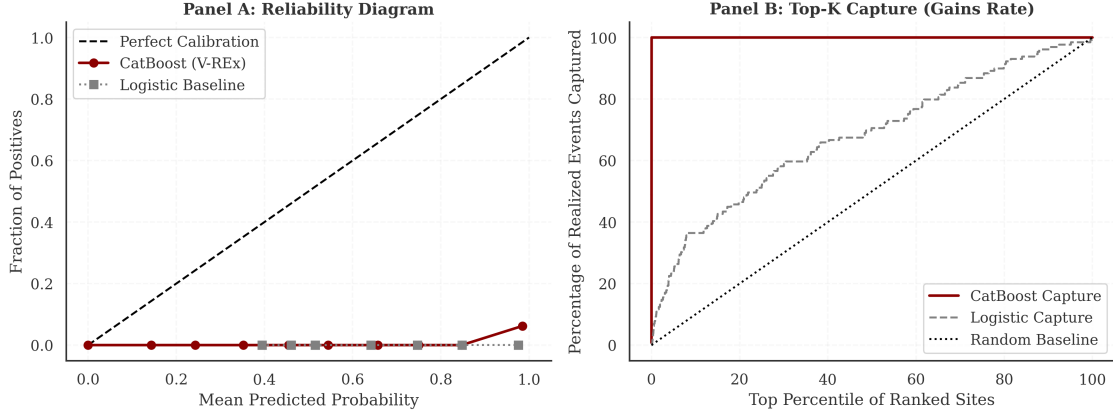
Figure 13: Stage A: Calibration reliability diagram (left) and top- K capture curve (right) for the Development Occurrence model (calculated using 10 equal-frequency bins to account for severe class imbalance).
