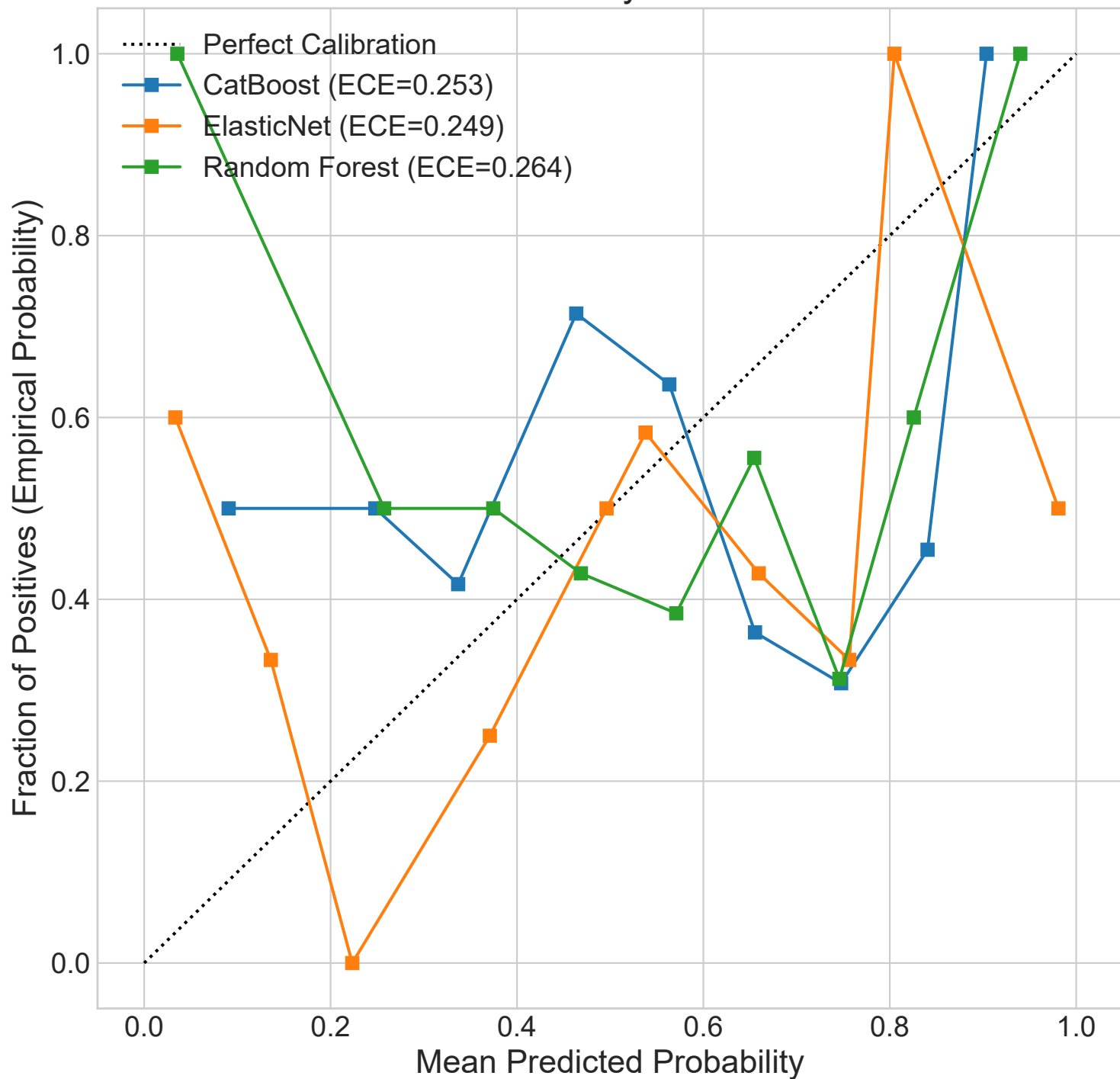
Model Reliability / Calibration
