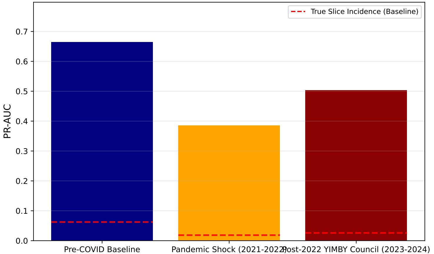
Out-of-Distribution Performance by Policy Period (Pre-Council Horizon)
