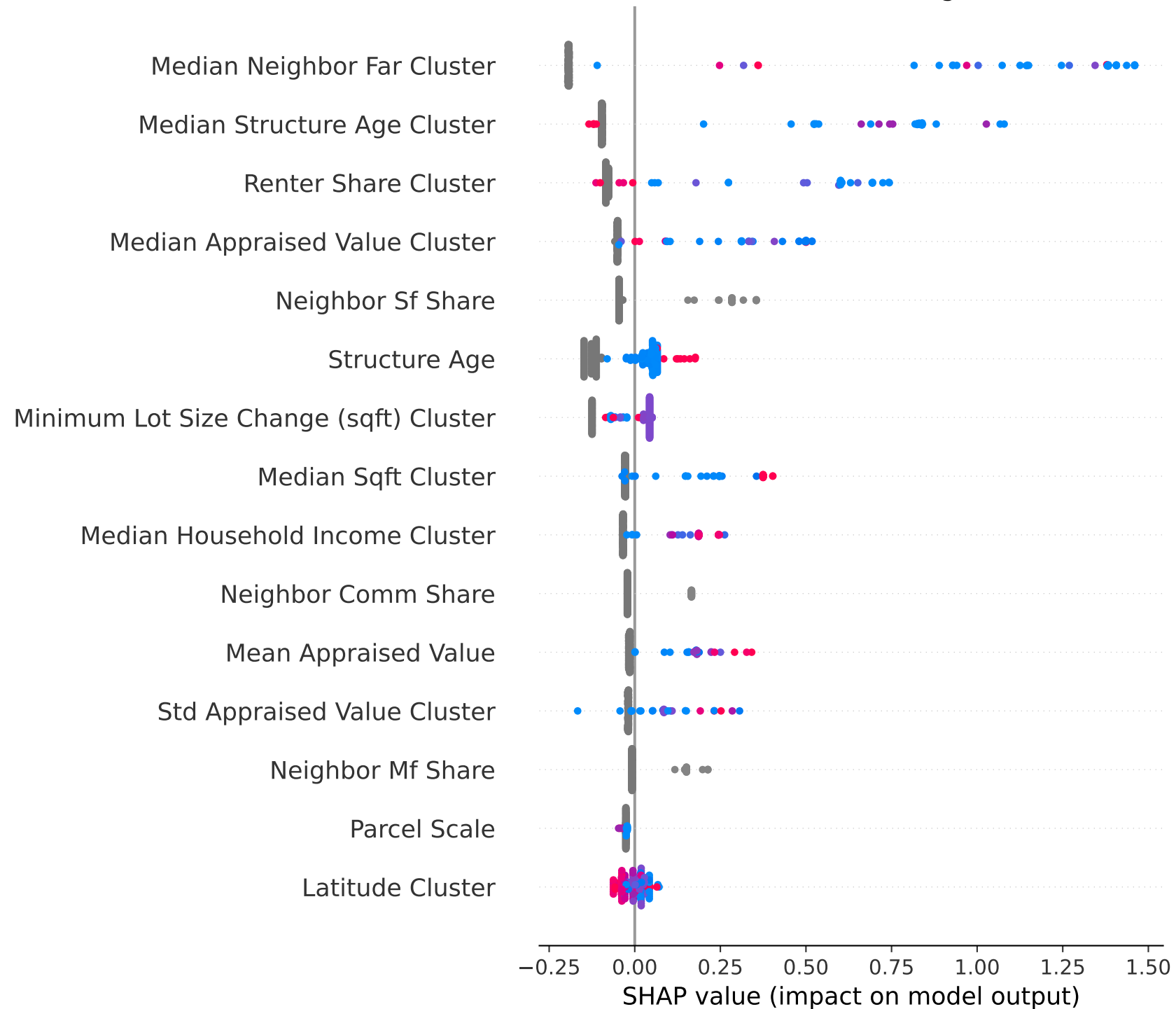
SHAP Feature Attribution (Filing Date Baseline)
