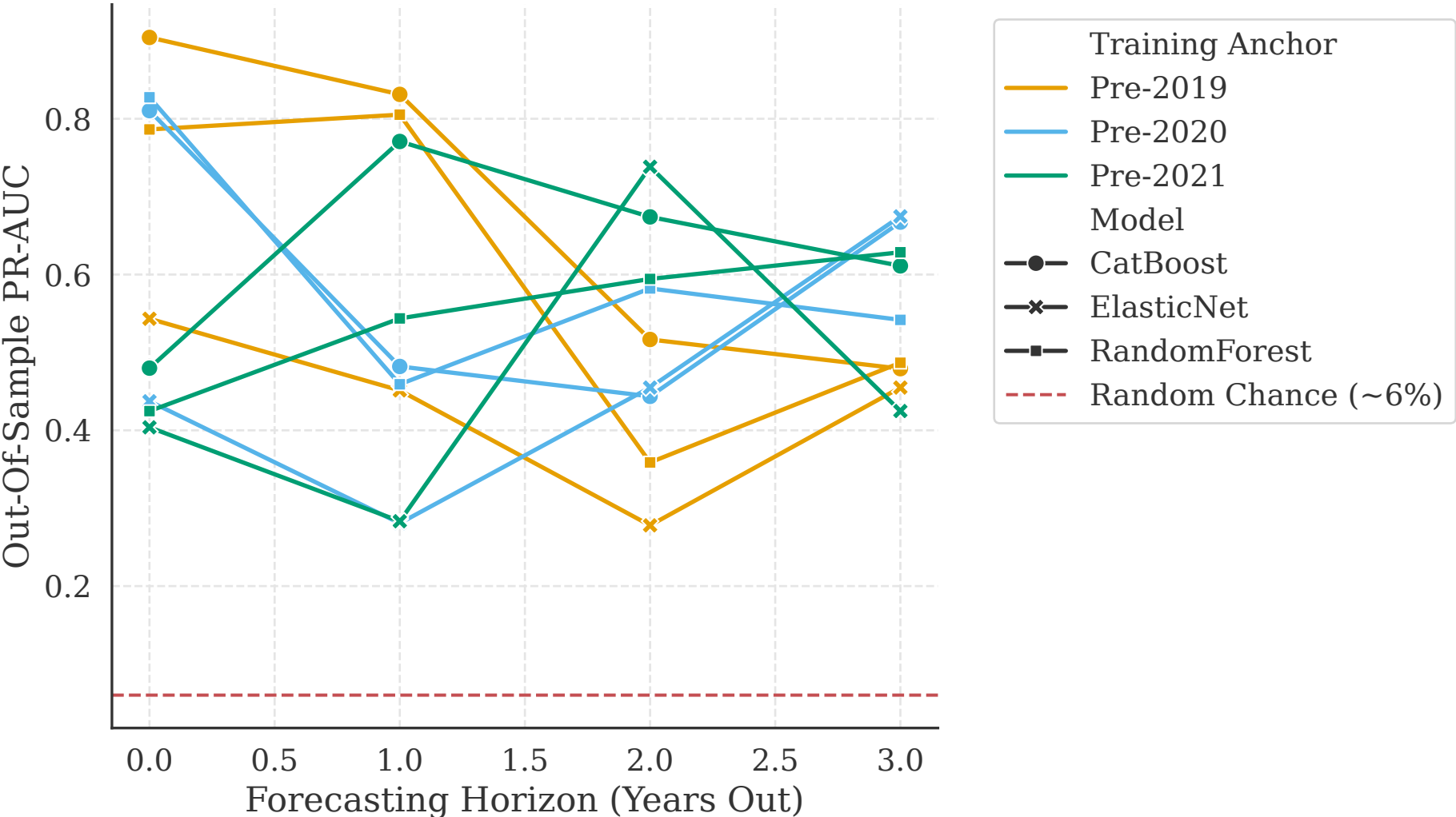
Predictive Temporal Drift (Model Rot over Time)
