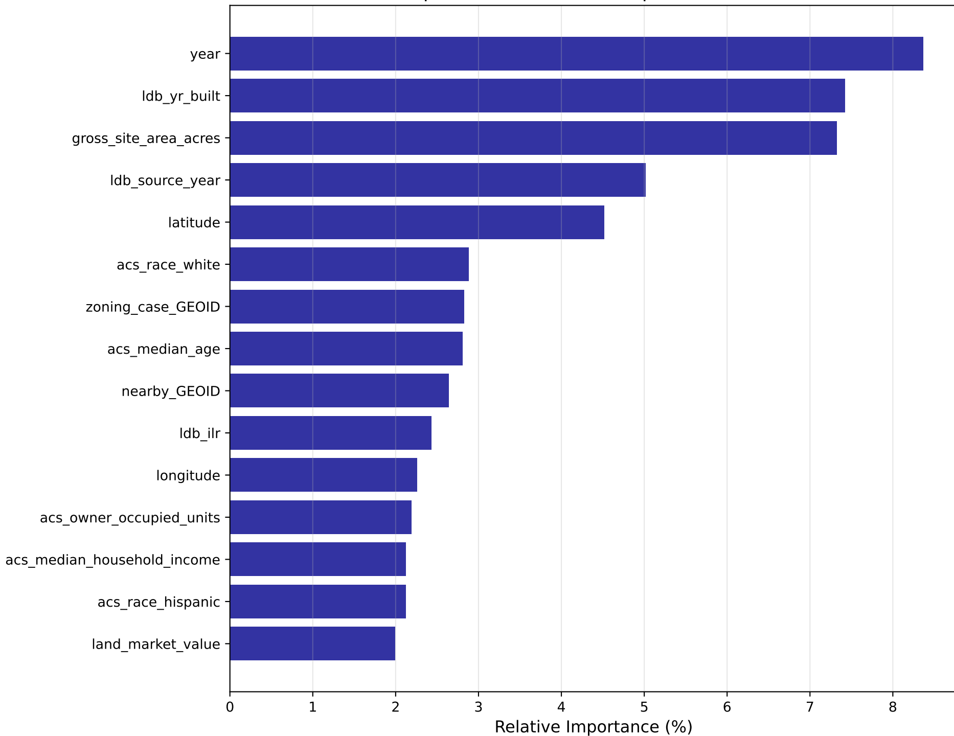
Top 15 Native Feature Importances (H0)
