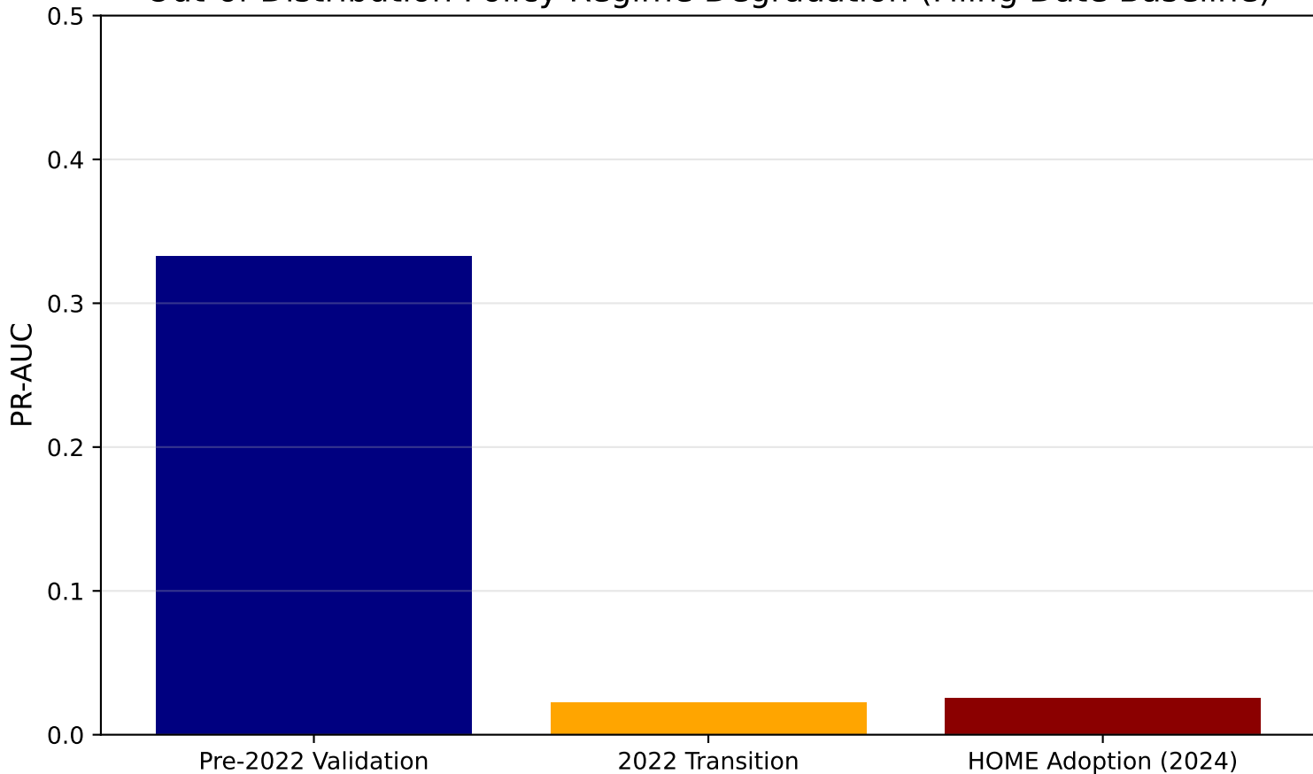
Out-of-Distribution Policy Regime Degradation (Filing Date Baseline)
