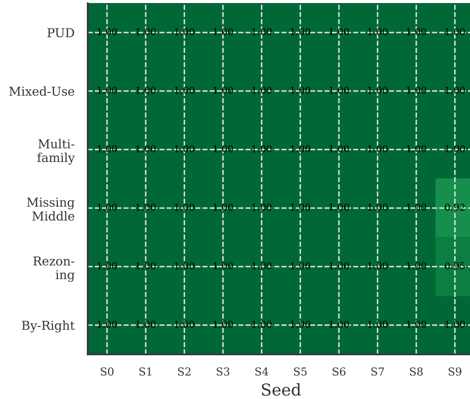
LightGBM
