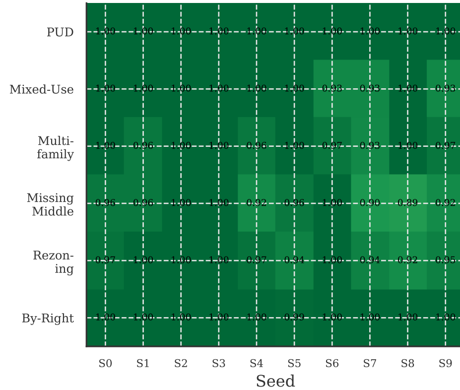
Random Forest
