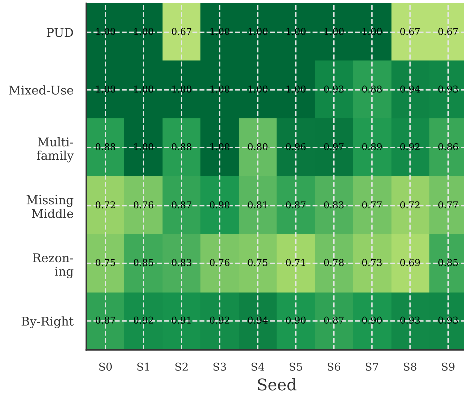
Logistic Regression
