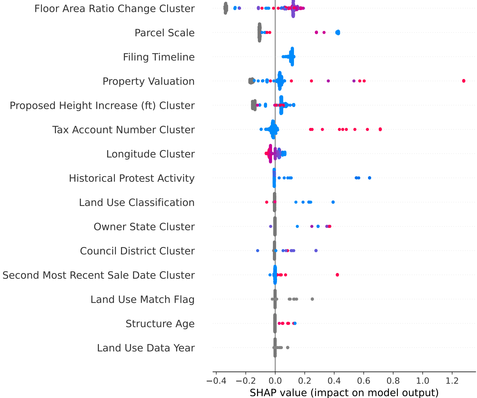
SHAP Feature Attribution (Filing Date Baseline)
