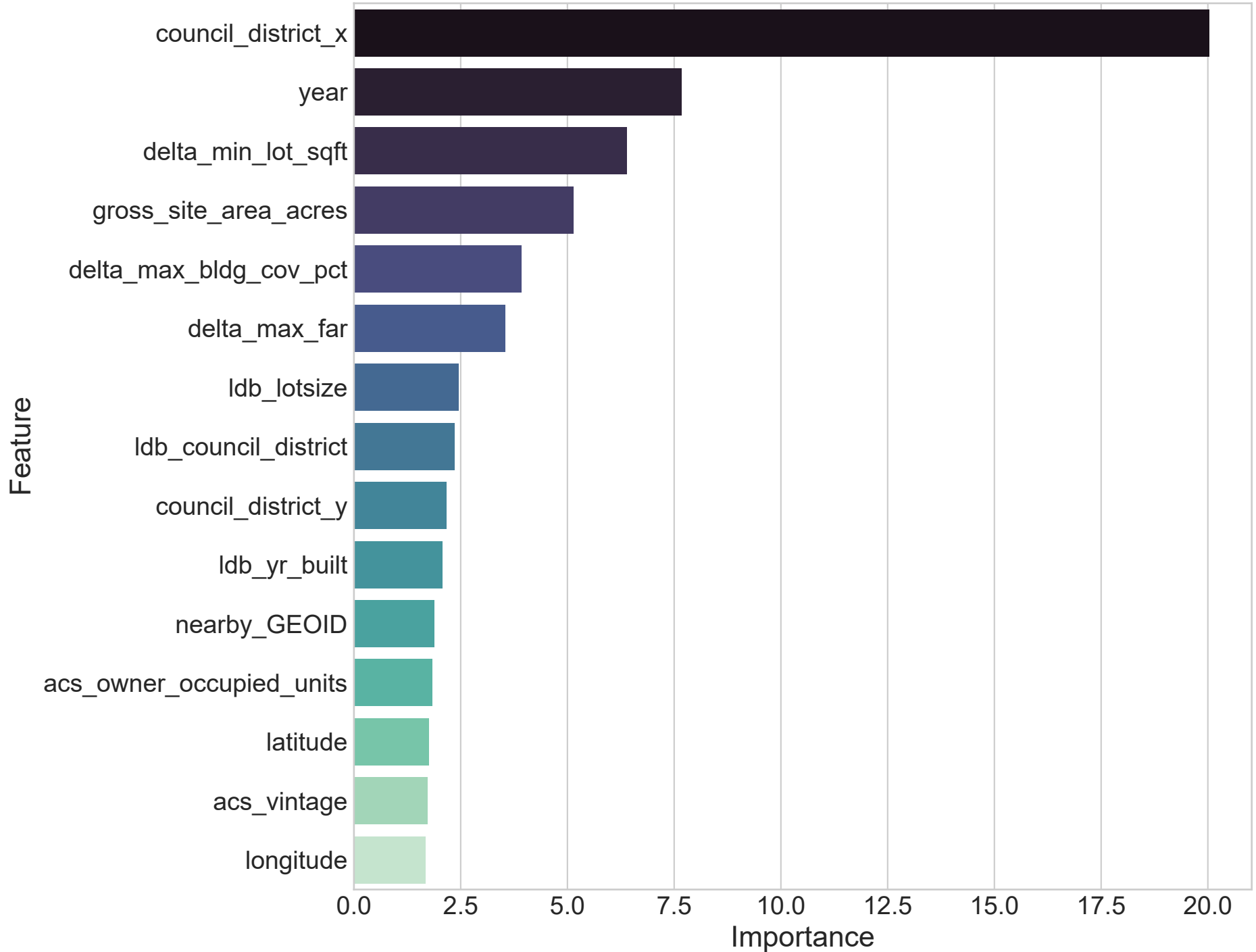
Primary Causal Signals (Permutation Importances)
