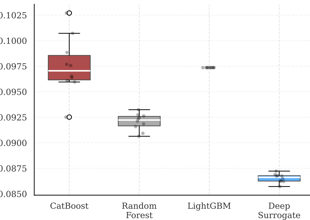
Stage A (Hazard) Brier Score
