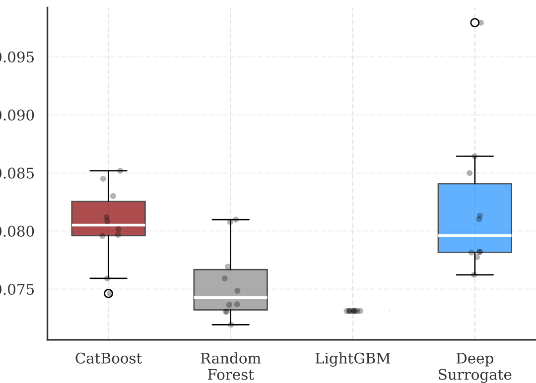
Stage A (Hazard) PR-AUC
