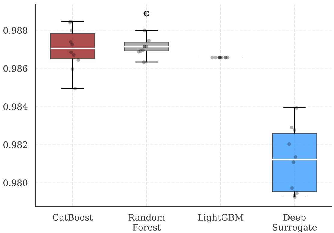
Stage C (Opposition) ROC-AUC
