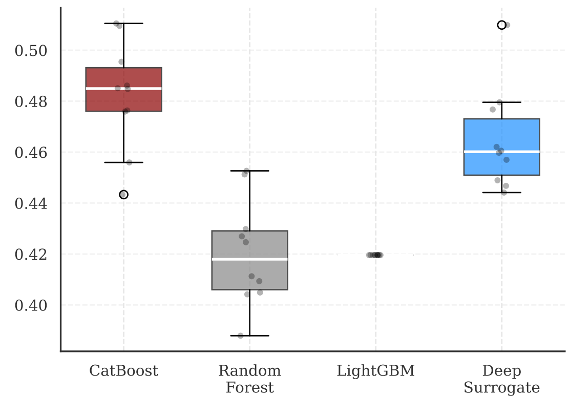
Stage A (Hazard) ROC-AUC
