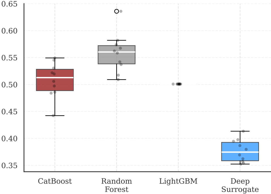
Stage C (Opposition) PR-AUC
