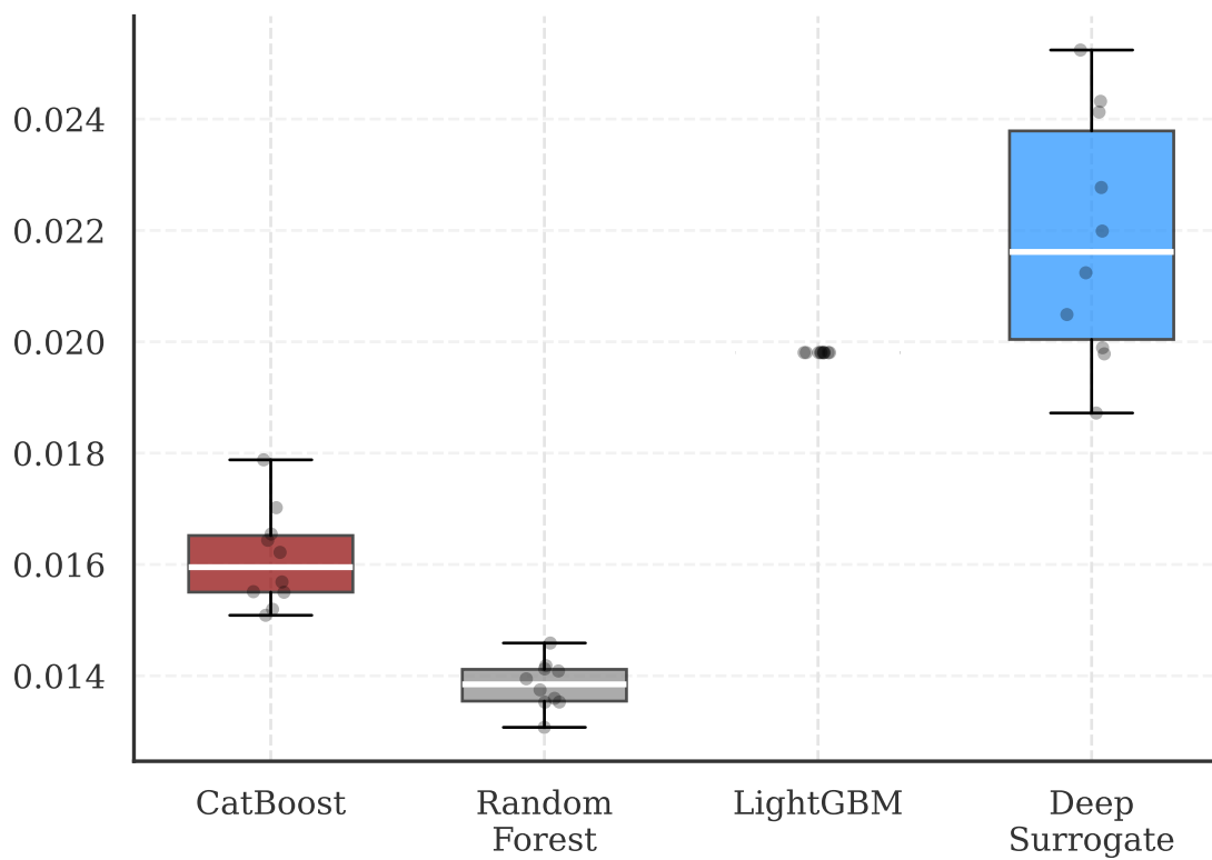
Stage C (Opposition) Brier Score
