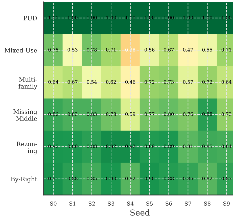
LightGBM
