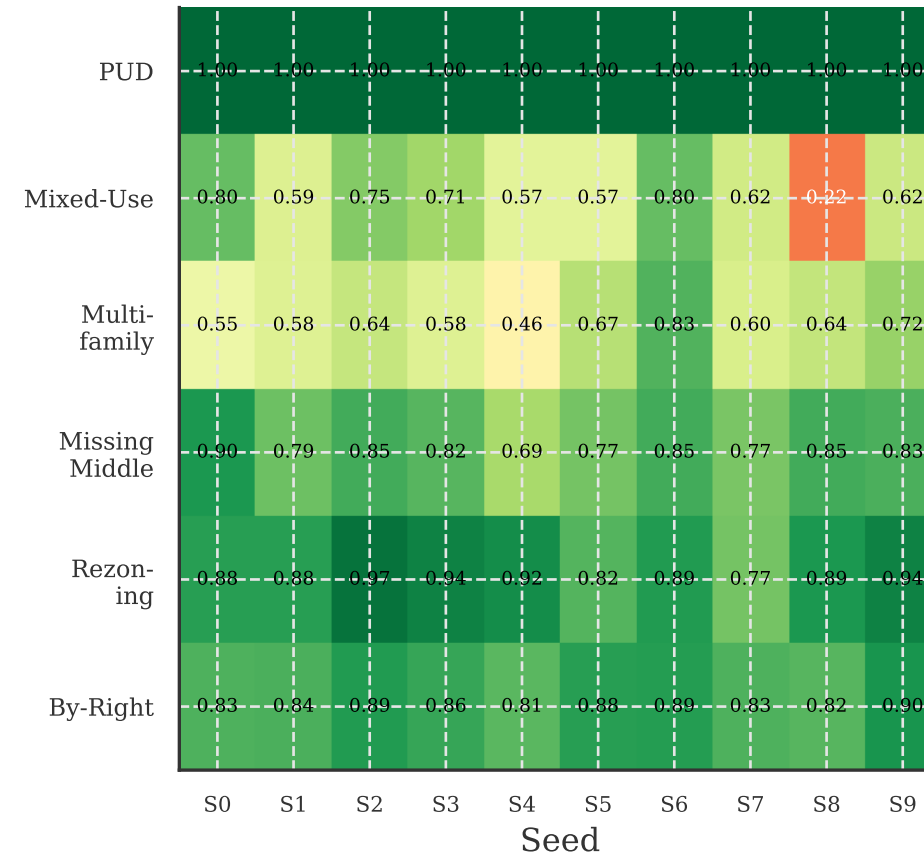
Random Forest
