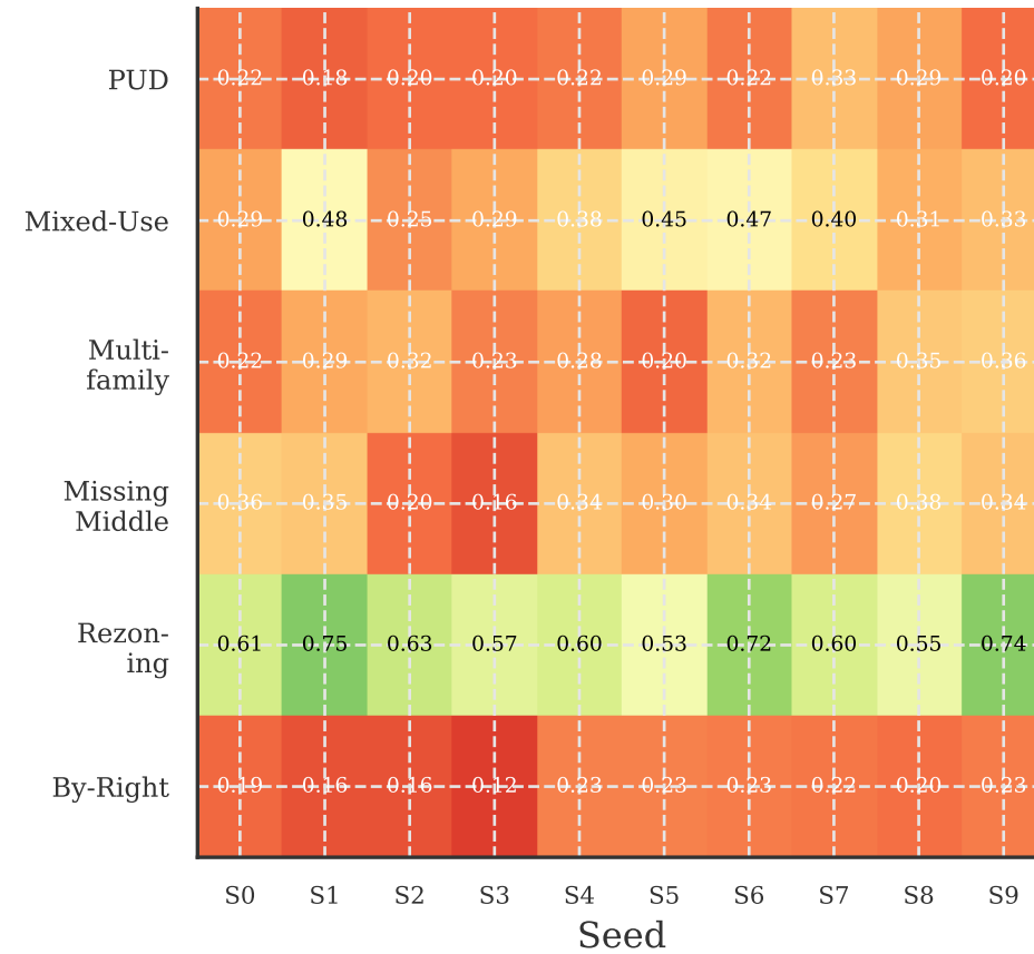
Logistic Regression
