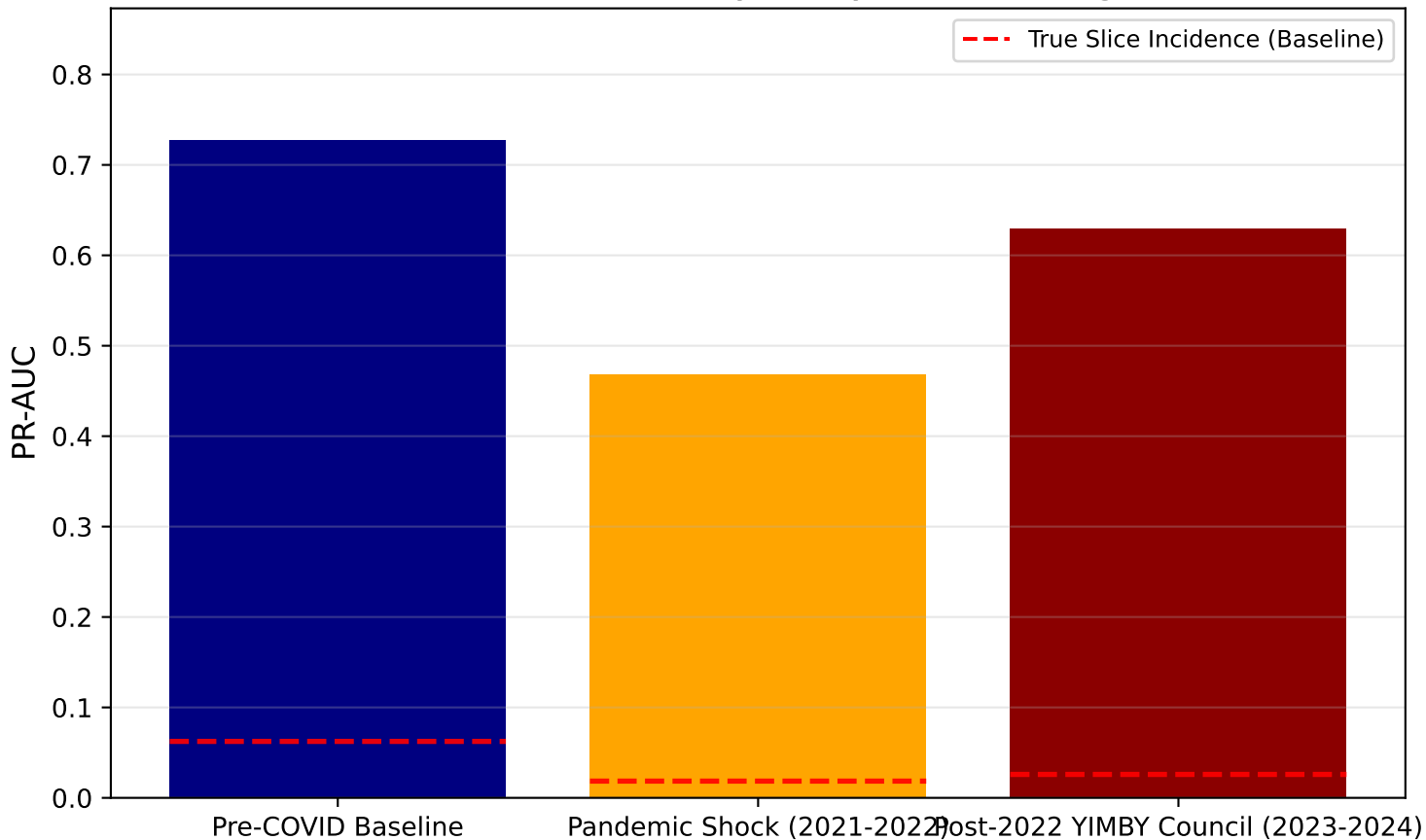
Out-of-Distribution Performance by Policy Period (Filing Date Baseline)
