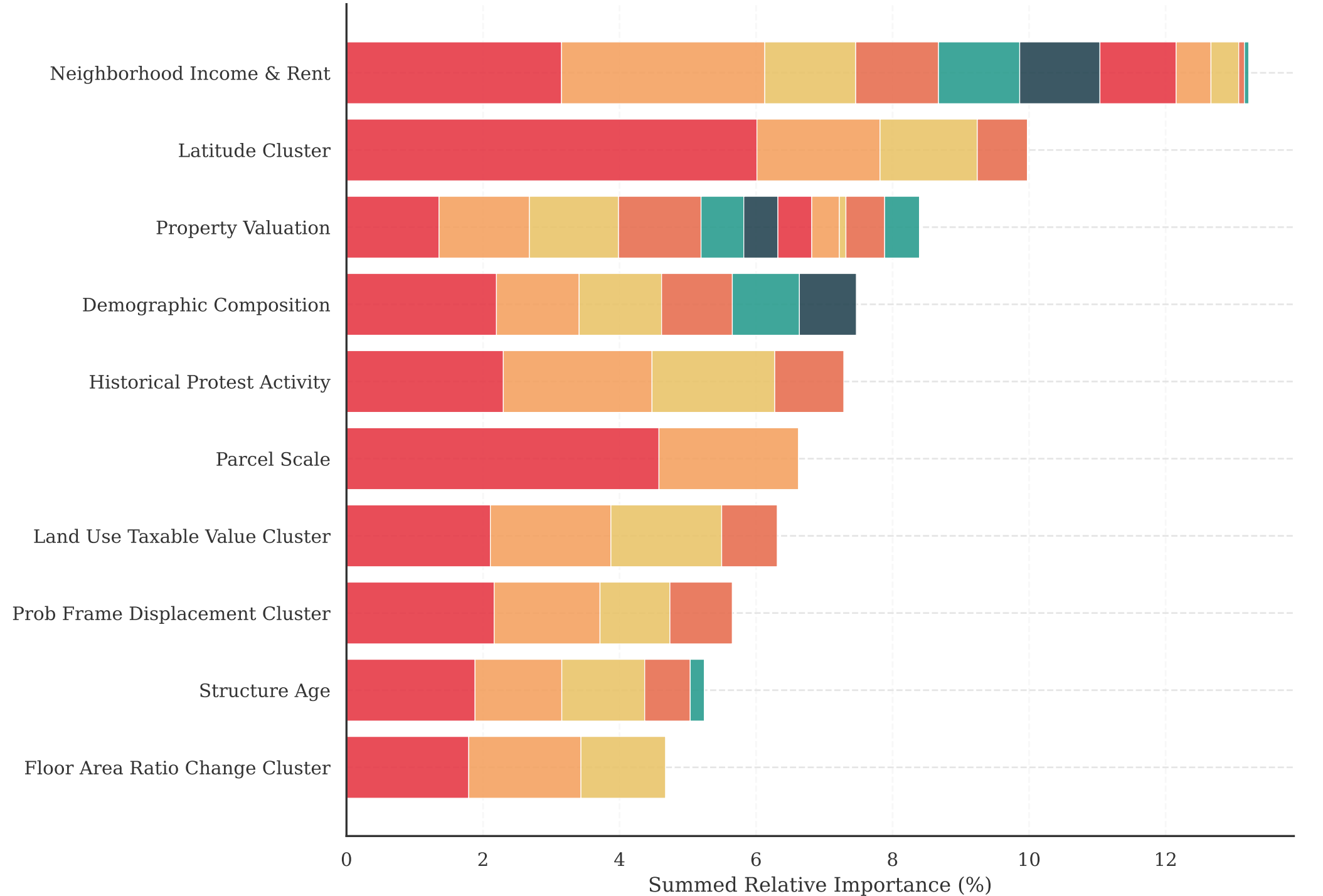
Top 10 Predictor Groups After Correlation Clustering (Pre-Council Horizon)
